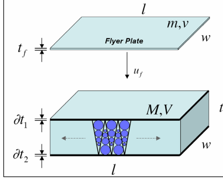
Figure 18. STC armor plate panel.
