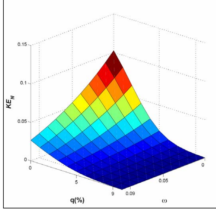
Figure 17. KE as a function of tapering and restitution for constant N = 20 and \Delta = 0.03\% .
