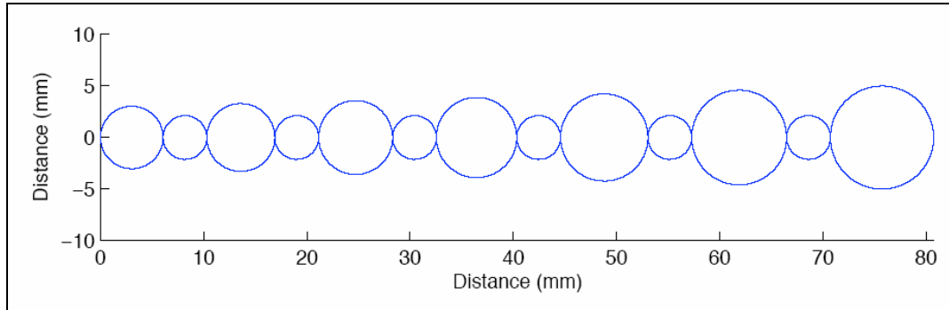
Figure 4. The decorated tapered chain: N = 13 , q = 8\% , f = 0.7 , L = 80.7 mm, and r_i = 5 mm.
