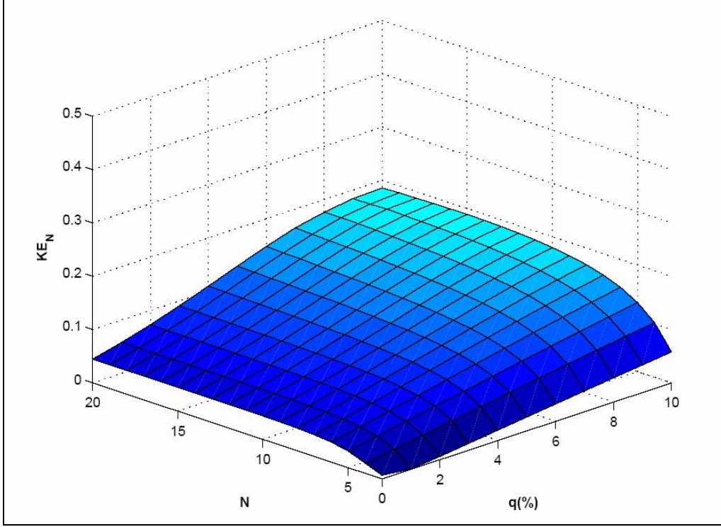
Figure 9. Difference plot of the lossless KE parameter spaces for the hard-sphere approximation (figure 2a) and numerical solution (7a). Note that the azimuthal view has been rotated 180° for clarity.
