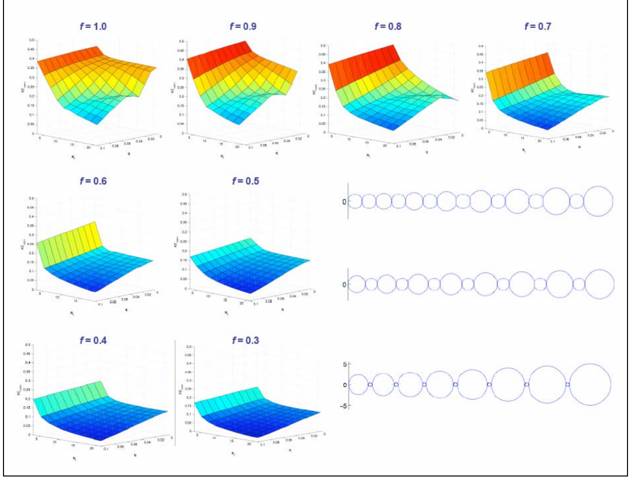
Figure 11. DTC numerical solution of KE(N, q, f) and sample DTCs for various f (inset). The scale is the same as that in figure 7.
