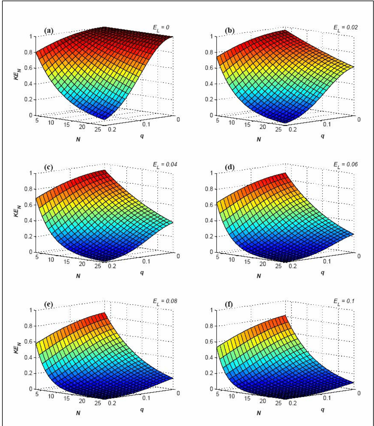
Figure 2. KE(N, q, E_L) parameter space for the STC hard-sphere approximation. N varies from 3 to 25 and q from 0% to 20%.
