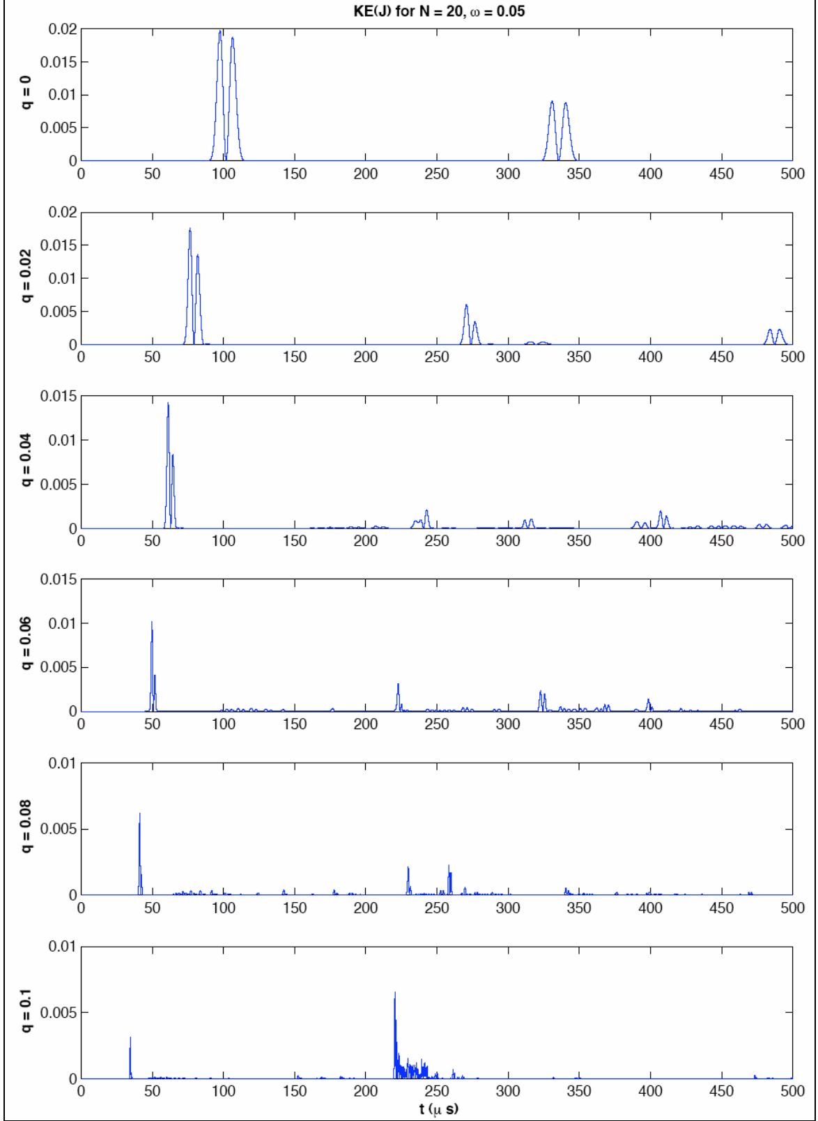
Figure 6. KE as a function of time for the smallest particle in a chain with N = 20 , \omega = 0.05 , and q = [0 : 0.02 : 0.1] . Each plot is evaluated for a different tapering with initial KE as 0.0838 J.
