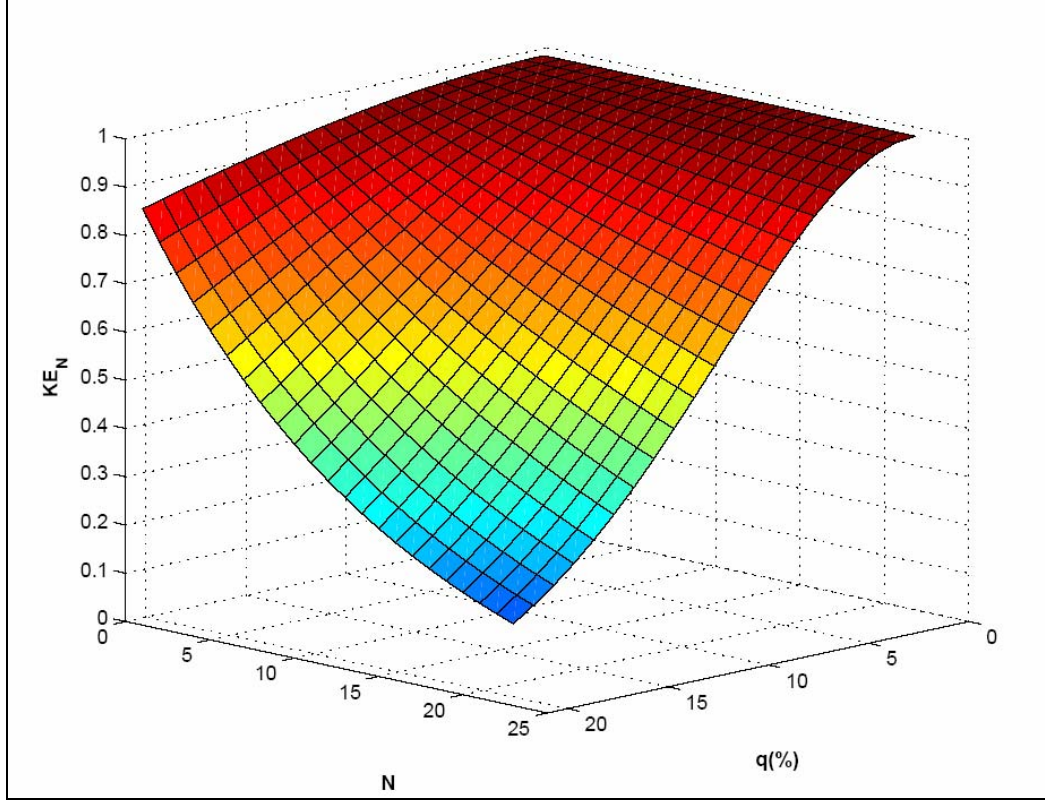
Figure 3. KE(N,q) parameter space for the STC hard-sphere approximation where the initial velocity is supplied to the smaller end of the chain.
