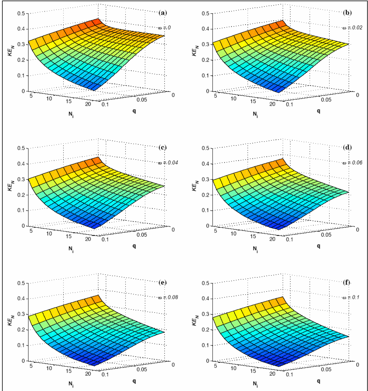
Figure 7. Numerical solution of KE(N, q) parameter space for constant \omega . Note that it would be very difficult and costly to produce a similar plot empirically. Each node on the surface represents a different TC and experiment.
