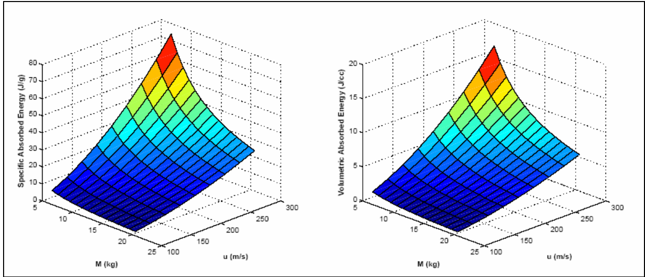
Figure 19. SAE and VAE as a function of M , the total STC armor panel mass, and u_f , the incident flyer plate velocity.
