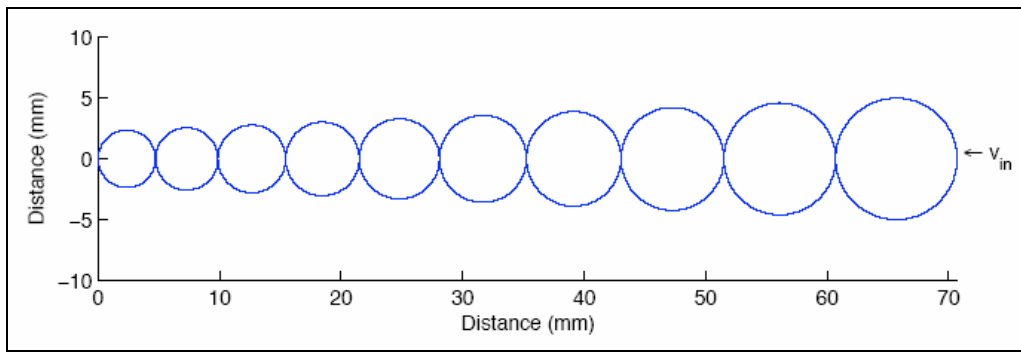
Figure 1. The simple tapered chain: N = 10 , q = 8\% , L = 70.7 mm, and r_i = 5 mm.
