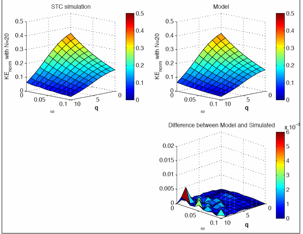
Figure 10. The simulated and modeled STC.
