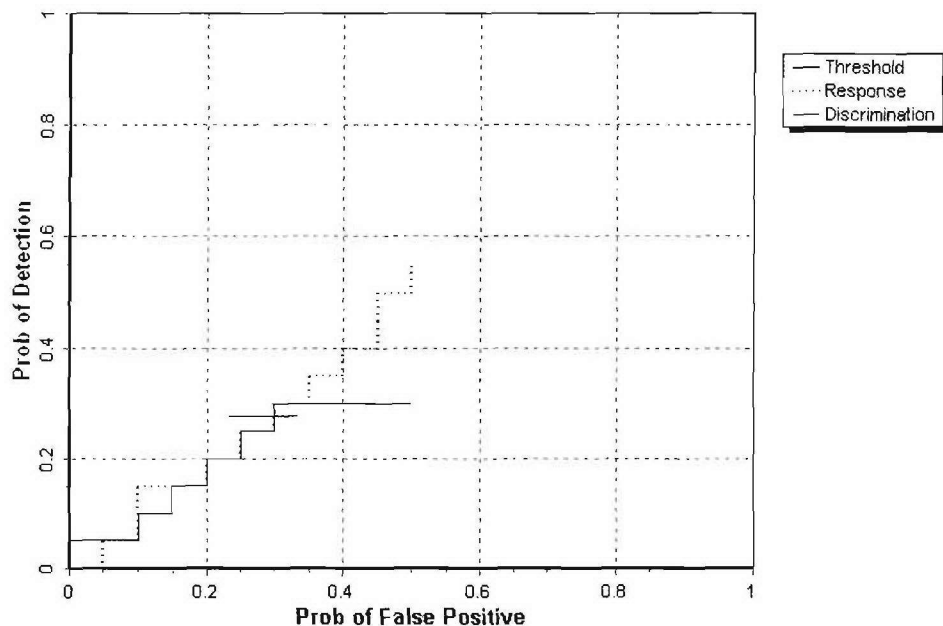
Figure 4. EM61-MKII/man-portable mogul probability of detection for response and discrimination stages versus their respective probability of false positive for all ordnance larger than 20 mm.
