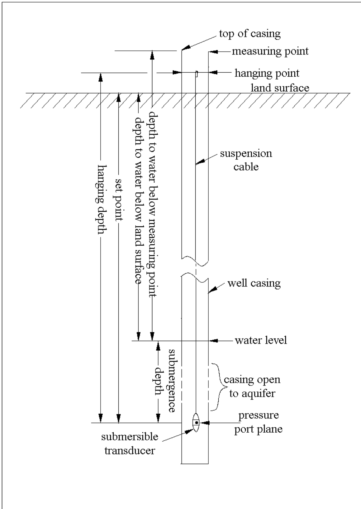
Figure 3. Submersible transducer in an observation well.
