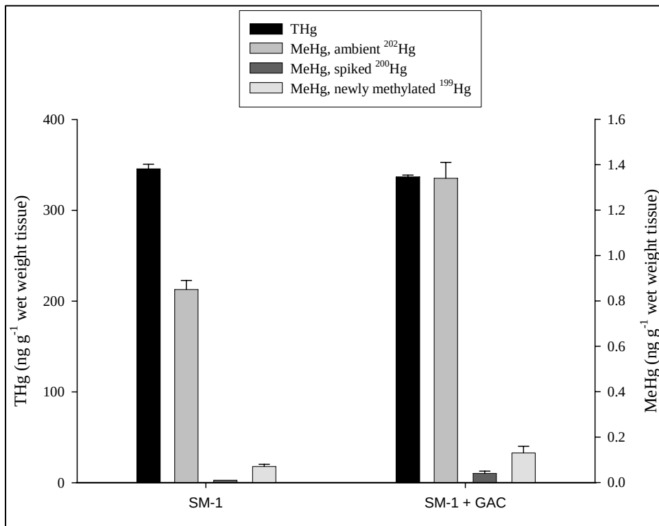
Figure 6-2. Effect of granular activated carbon on sediment pool sizes of legacy 202 Hg, spikes \text{Me}^{200}\text{Hg} , and newly methylated \text{Me}^{199}\text{Hg}
