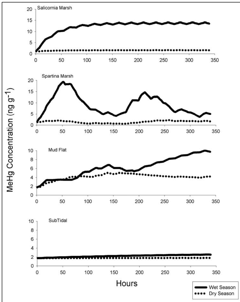
Figure 7-8. Simulated MeHg concentrations in surface sediments of four spatial areas
