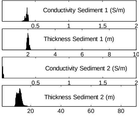
Fig. 2. Marginal PPDs estimated from single frequency (30kHz) data with a SNR of 30dB.
