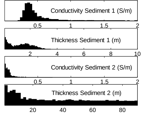
Fig. 3. Estimated marginal PPDs from 4 sensors and 9 frequencies data with a SNR of 15dB and 30m separation distance.
