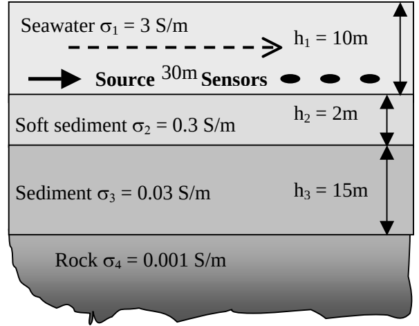
Fig. 1. Geometry of the marine environment.
