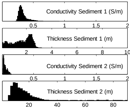
Fig. 5. Estimated marginal PPDs from multi-frequency (10 – 30 kHz) data with 15dB SNR and 50m separation distance.
