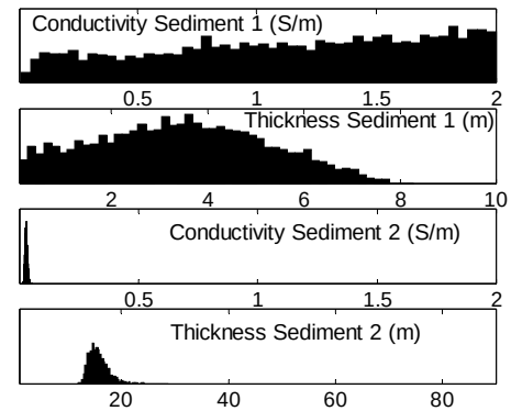
Fig. 4. Estimated marginal PPDs from 10 sensors single frequency data with a SNR of 15dB and 30m separation distance.
