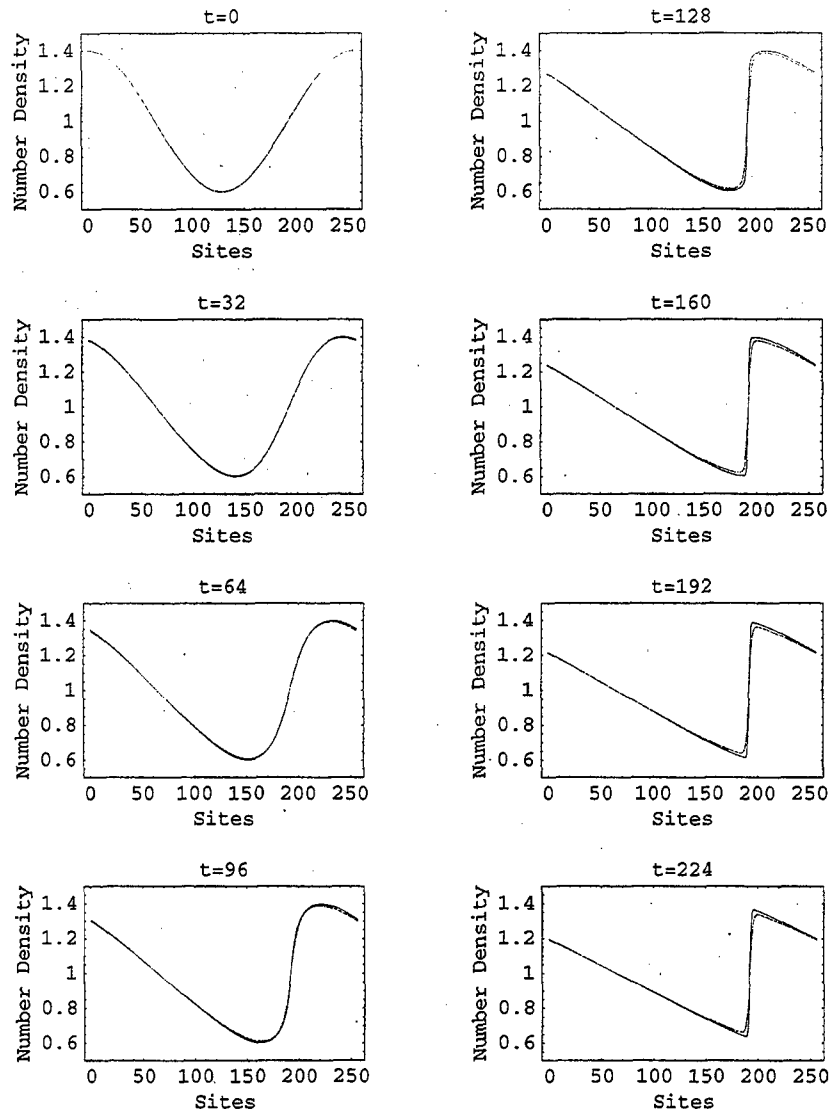
Figure 2: Development of a shock front in the number density field after the system was initialized with a sinusoidal profile on a L = 256 site lattice. Agreement between the numerical data (blue curve) and the analytical solution (red) curve is apparent. However, the analytical solution appears to depart from the numerical solution at later times when a steep shock front is fully formed. The edges of the analytical solution are smooth compared to the sharp edges of the numerical simulation.
