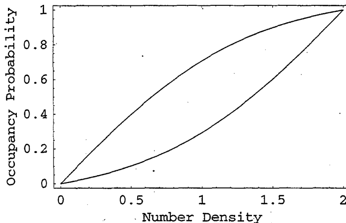
Figure 1: A plot of the occupancy probabilities of the two on-site qubits versus the number density at that site. The upper curve is f_1^{\text{eq}} and the lower curve is f_2^{\text{eq}} as specified by (38). In a quantum lattice gas, the occupancy probabilities can be different while the system nevertheless obeys a detailed-balance condition. The abscissa and ordinate are both non-dimensional probability values.
