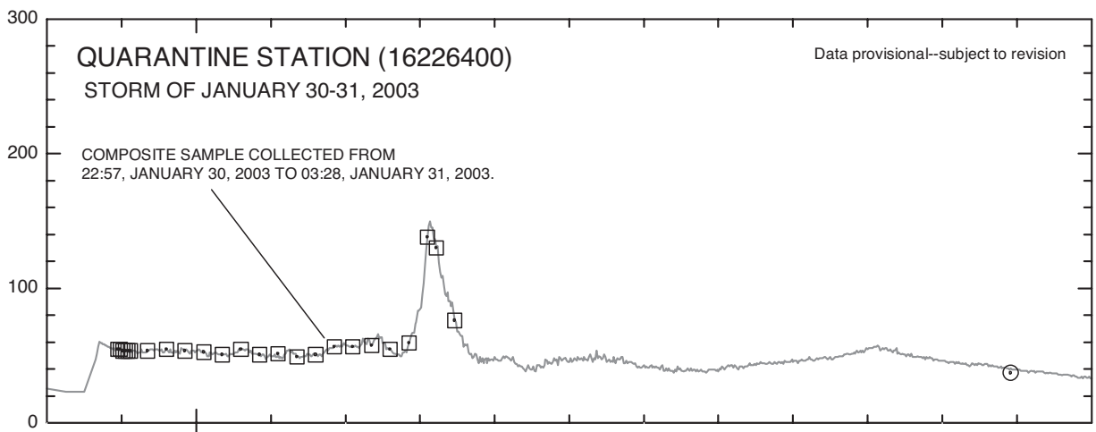
Figure 11. Stream discharge at Quarantine station (16226400) for January 1 to March 31, 2003; detail of the 4-day period from January 30, 2003 to February 2, 2003; and detail of the 14-hour period from 22:00 January 30, 2003 to 12:00 January 31, 2003, Oahu, Hawaii.
