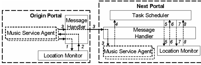
Figure 4: Portal to Portal Interactions
