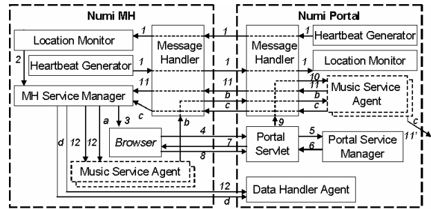
Figure3: Mobile Host to Service Portal Interaction
