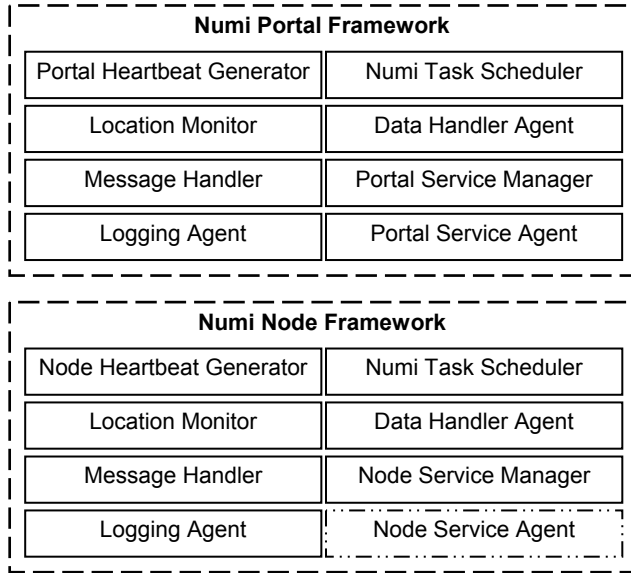
Figure2: Numi Portal and Mobile Host Platforms
