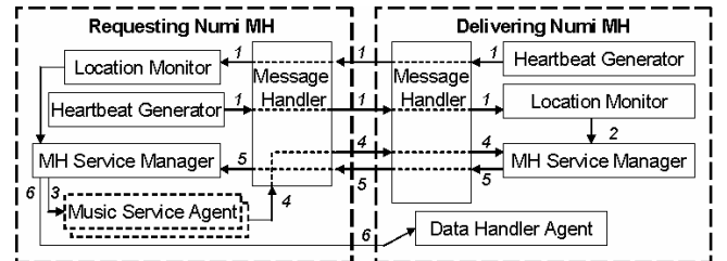
Figure 5: Mobile Host to Mobile Host Interactions
