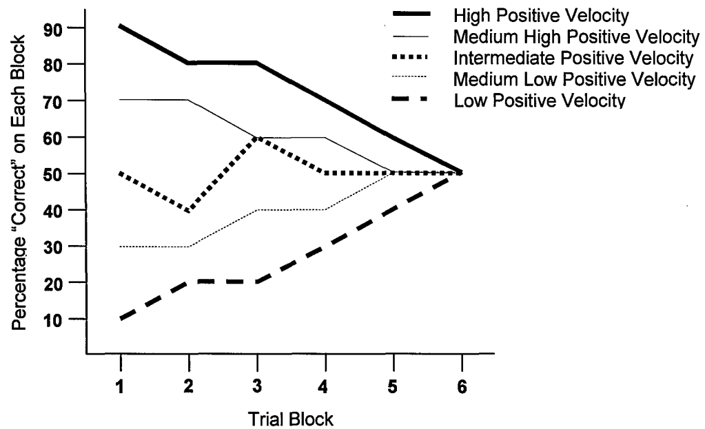
Figure 2. Lawrence et al.'s (2002) velocity feedback conditions.
