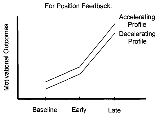
Figure 9a. Hypothesized feedback frame x performance profile x time interaction for position feedback.
