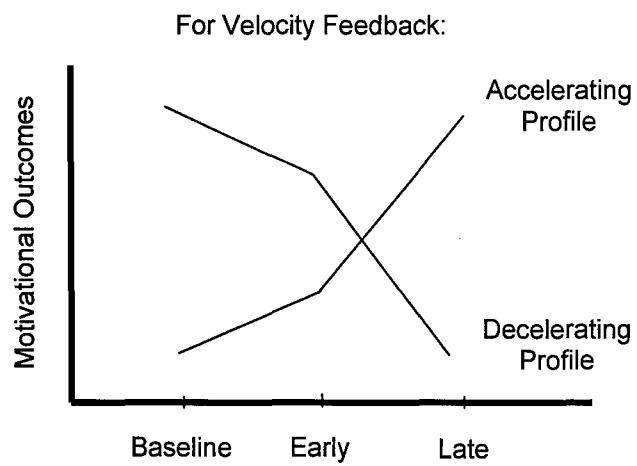
Figure 9b. Hypothesized feedback frame x performance profile x time interaction for velocity feedback.
