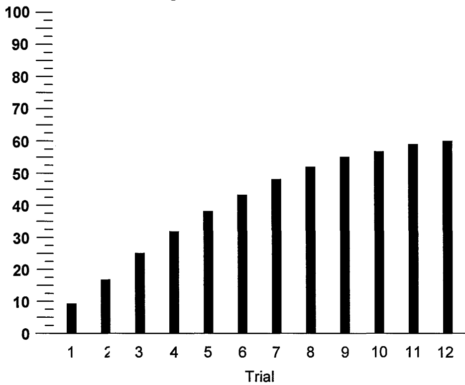
Decelerating Performance Profile with Position Feedback
