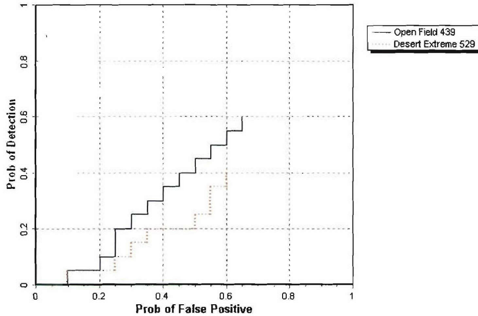
Figure 8. MAG TM-4/sling P_d^{\text{res}} versus the respective P_{fp} for ordnance larger than 20 mm.
