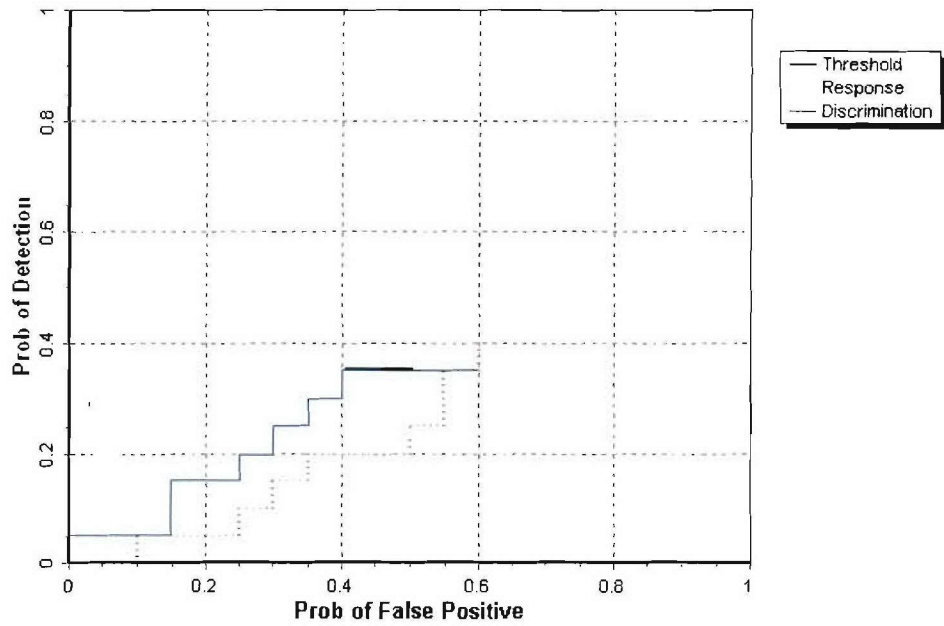
Figure 4. MAG TM-4/sling desert extreme probability of detection for response and discrimination stages versus their respective probability of false positive for all ordnance larger than 20 mm.
