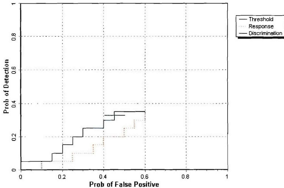
Figure 2. MAG TM-4/sling desert extreme probability of detection for response and discrimination stages versus their respective probability of false positive over all ordnance categories combined.
