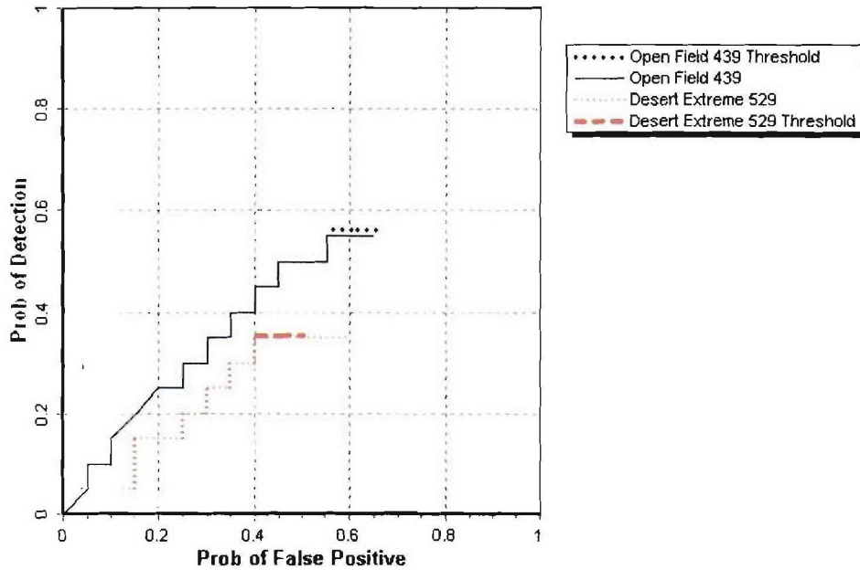
Figure 9. MAG TM-4/sling P_d^{\text{disc}} versus the respective P_{fp} for ordnance larger than 20 mm.
