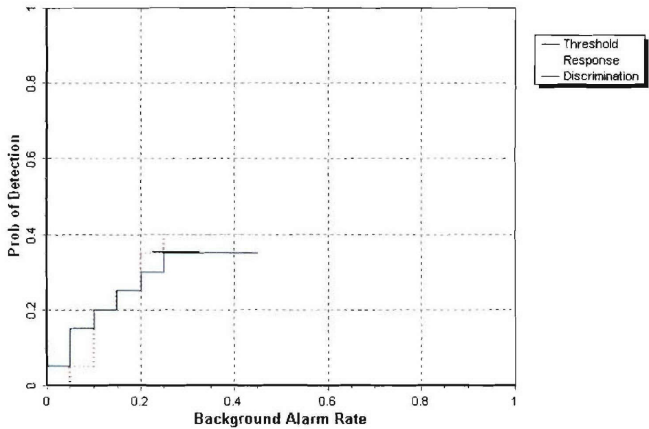
Figure 5. MAG TM-4/sling desert extreme probability of detection for response and discrimination stages versus their respective probabilities of background alarm for all ordnance larger than 20 mm.
