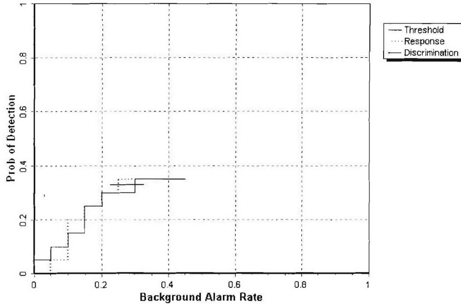
Figure 3. MAG TM-4/sling desert extreme probability of detection for response and discrimination stages versus their respective probability of background alarm over all ordnance categories combined.
