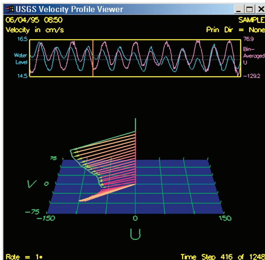
Figure 3. A three-dimensional profile displayed by the Velocity Profile Viewer.
