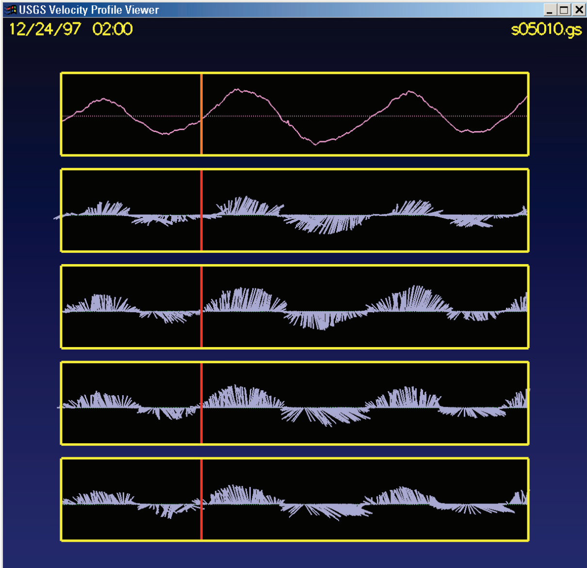
Figure 36. The Bin Graph View of the Velocity Profile Viewer showing tidal velocity stick plots on a blue background. Graphs for bins 17-20 are shown below the Main Graph. The time span shows about 1.5 tidal cycles.
