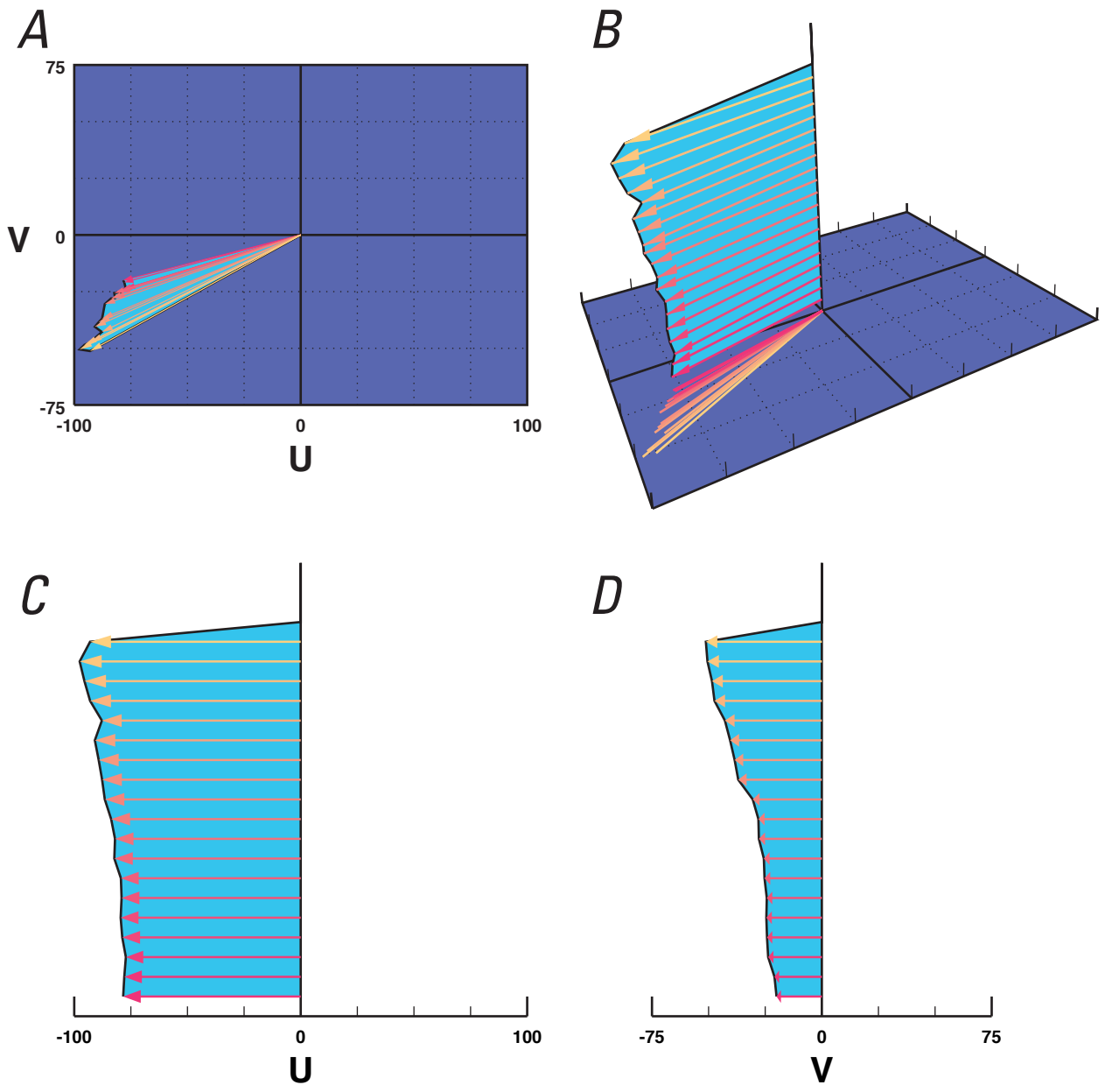
Figure 41. Example showing color PostScript output from the Velocity Profile Viewer showing a profile with arrows, a surface, and grid lines on the base. The four views shown are (A) top; (B) perspective; (C) front; and (D) side. Arrows, the profile surface, grid lines, axis labels, and the date and location text are shown. The units and principal direction text are not shown.
