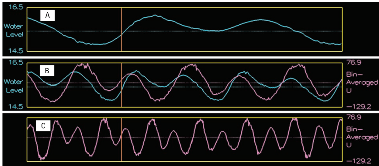
Figure 27. The Main Graph of the Velocity Profile Viewer showing variations in plots of water level and bin-averaged U velocity.
