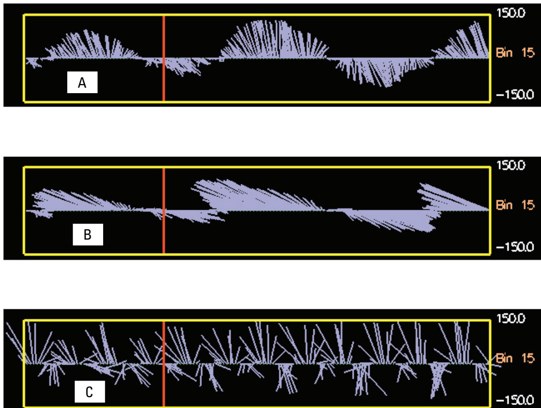
Figure 9. Three different displays of the same bin from the Bin Graph View in the Velocity Profile Viewer. The sticks are (A) easy to discern; (B) skewed because the principal direction is not set; (C) sparse because the time span has been expanded.
