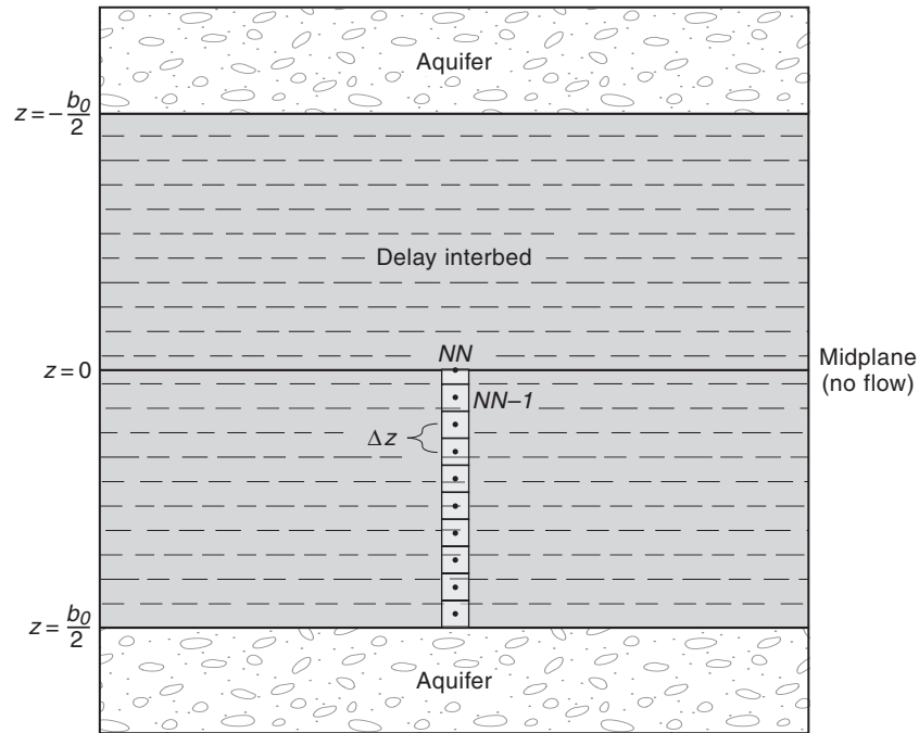
Figure 3. Finite difference cells and nodes used in numerical approximation given by equation 11. The symmetry of the problem is exploited by computing the heads at nodes for only one-half of the interbed. z is the vertical coordinate referenced to a datum, b is the interbed thickness, NN is the number of finite-difference nodes used to discretize the interbed half-thickness, \Delta z is the spacing between finite-difference nodes.
