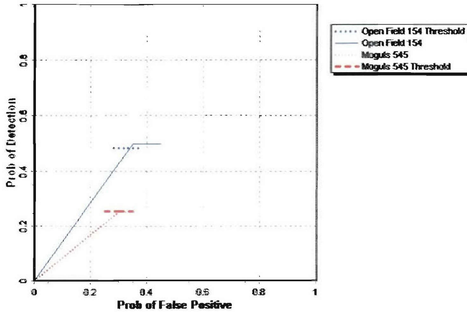
Figure 9. TM-5 EMU/hand held sling P_d^{\text{disc}} versus the respective P_{\text{fp}} for ordnance larger than 20 mm.
