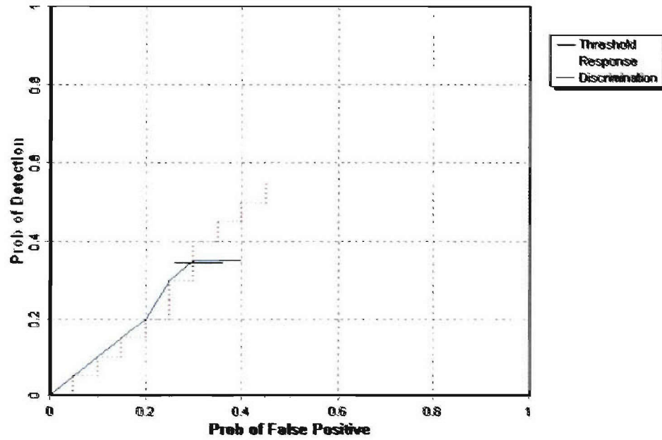
Figure 4. TM-5 EMU wooded area probability of detection for response and discrimination stages versus their respective probability of false positive for all ordnance larger than 20 mm.
