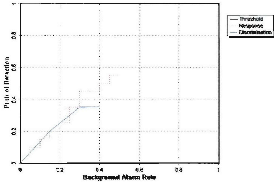
Figure 5. TM-5 EMU wooded area probability of detection for response and discrimination stages versus their respective background alarm rate for all ordnance larger than 20 mm.
