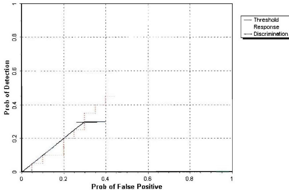
Figure 2. TM-5 EMU wooded area probability of detection for response and discrimination stages versus their respective probability of false positive over all ordnance categories combined.
