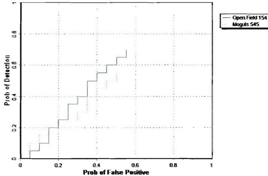
Figure 8. TM-5 EMU/hand held sling P_d^{res} versus the respective P_{fp} for ordnance larger than 20 mm.
