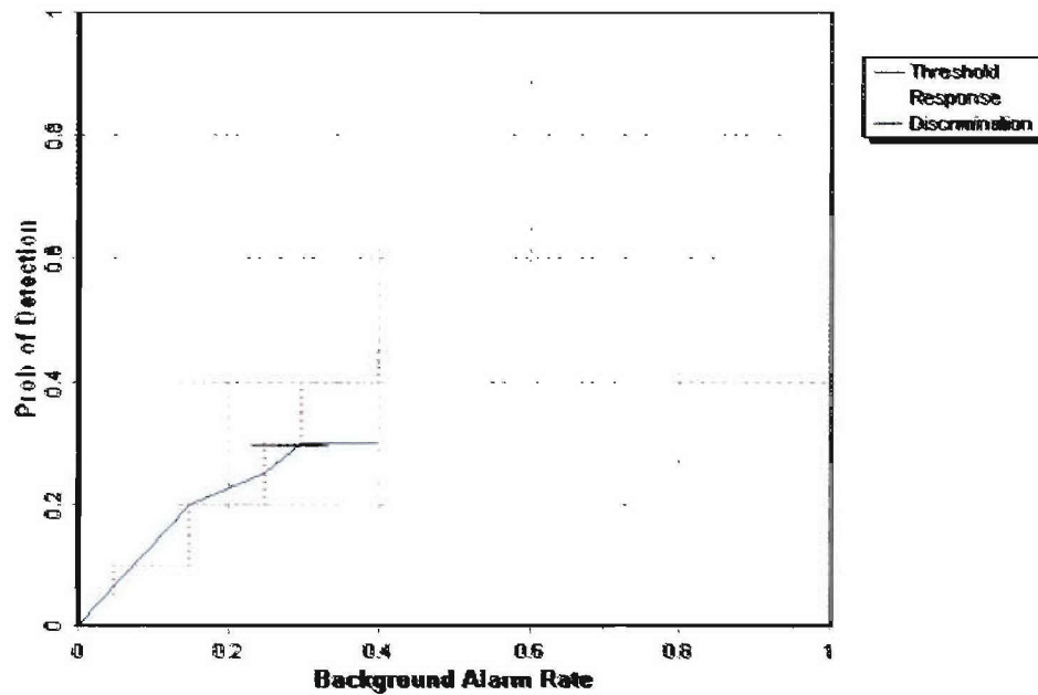
Figure 3. TM-5 EMU wooded area probability of detection for response and discrimination stages versus their respective background alarm rate over all ordnance categories combined.
