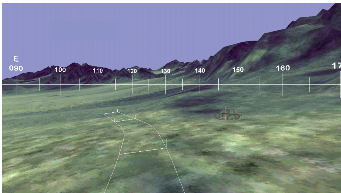
Figure 6.4.3. Cueing reticle, course deviation indicator, and heading tape superimposed in the high detail scene.
