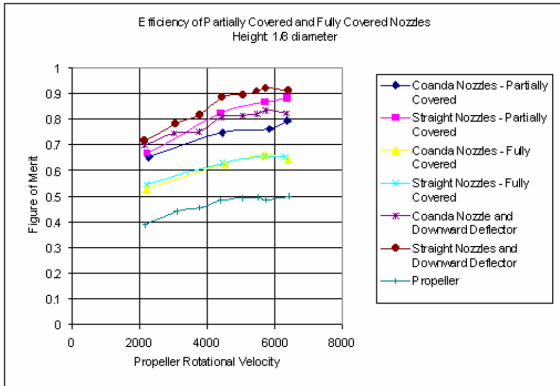
Figure 38: Efficiency vs. propeller rotational velocity. Covered and fully covered nozzles comparison with open nozzles configurations at 1/8 diameter height
