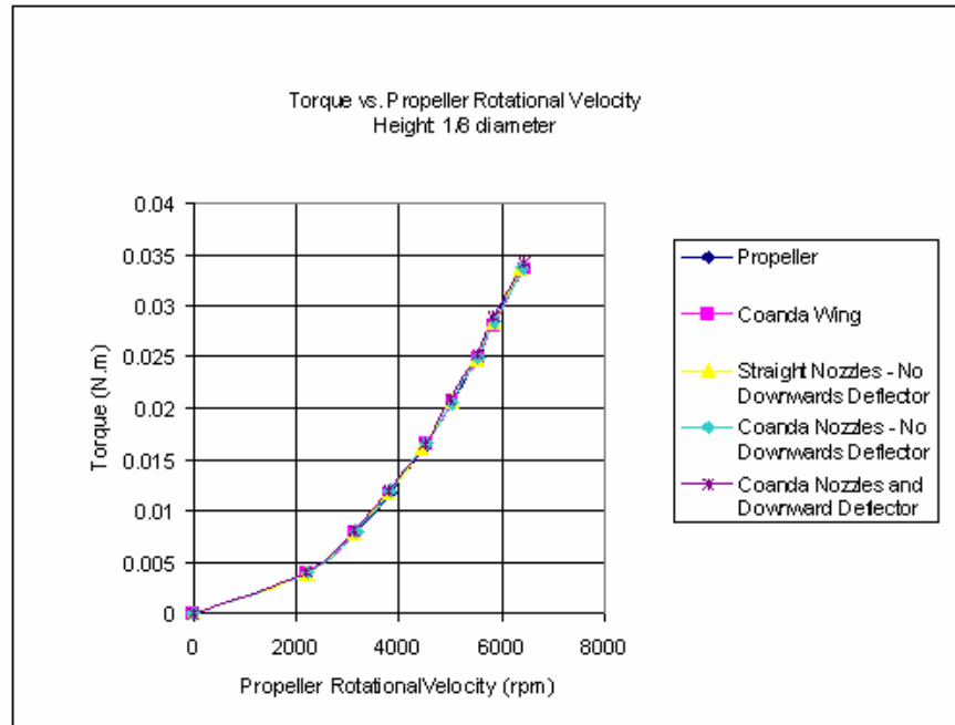
Figure 59: Torque vs. propeller rotational velocity. 1 st group of tests, 1/8 diameter height
