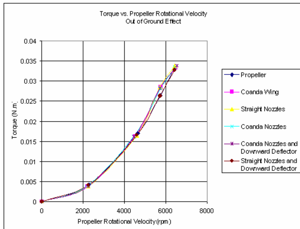
Figure 22: Torque vs. propeller rotational velocity out of ground effect
