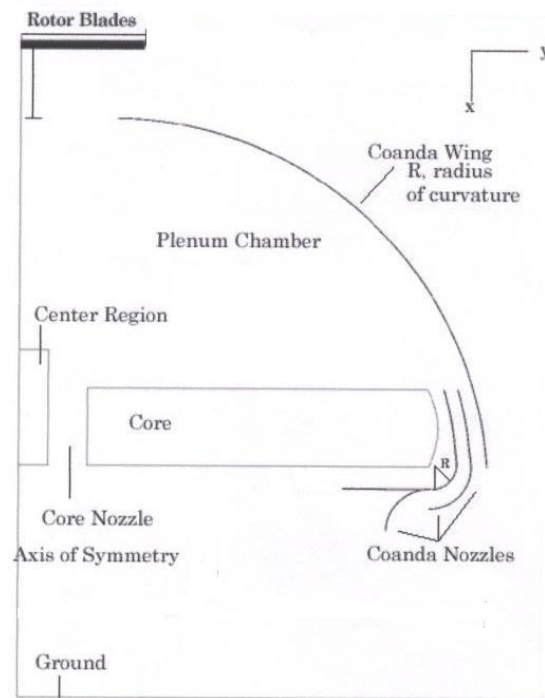
Figure 13: Half a cross sectional view of Kelleher's third model (4)
