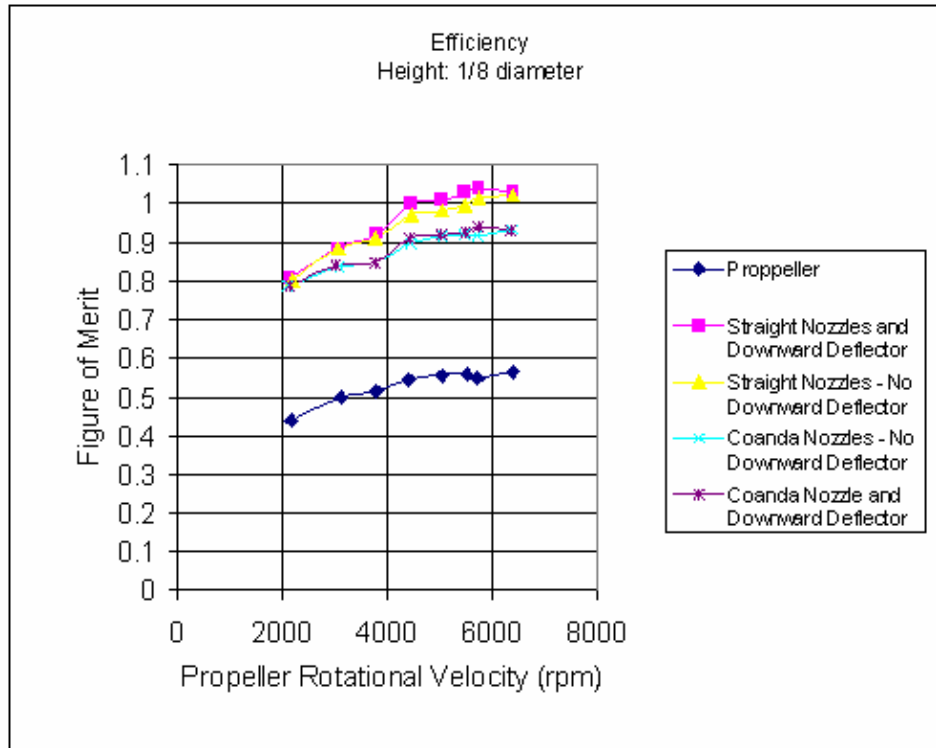
Figure 28: Efficiency vs. propeller rotational velocity at 1/8 diameter height
