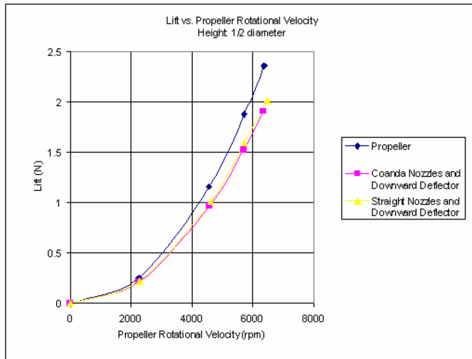
Figure 25: Lift vs. propeller rotational velocity at 1/2 diameter height
