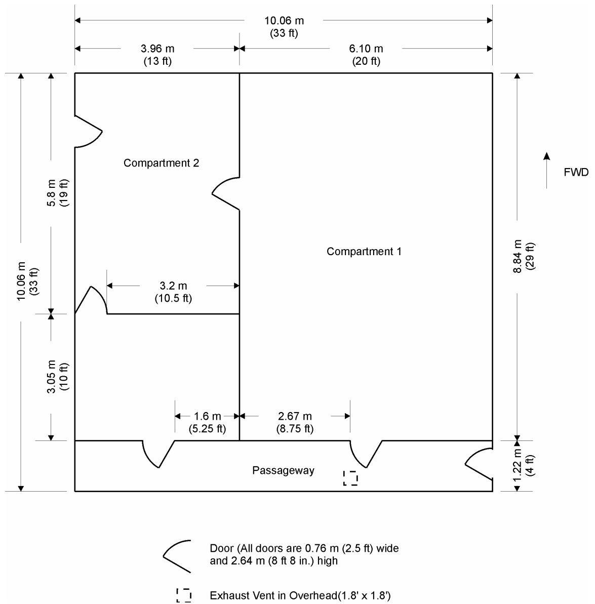
Fig. 1 — Compartment layout within test facility
