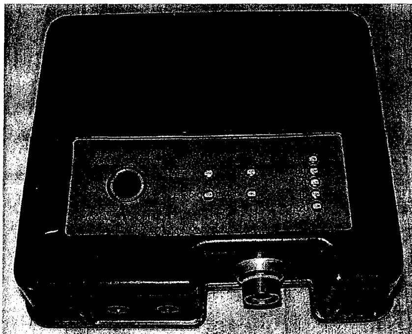
Figure 9. First-pass case design. This two-piece design holds the AC-DC converter's heat-sink against the inside wall of the case. The charger's PCB location utilizes a PCB-mounted bulkhead connector, rather than cable/wires between the PCB and the connector.
