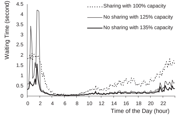
Figure 7. Average waiting times with and without resource sharing for different processing capabilities of the proxy server.
