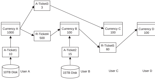
Figure 1. Use of tickets and currencies to express sharing agreements.
