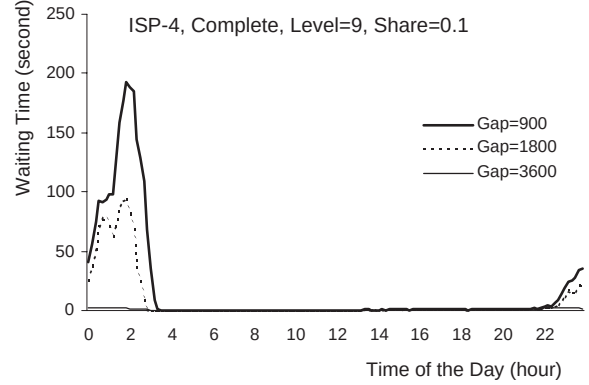
Figure 6. Average waiting time per request with resource sharing for different “gap” times (skew) between the proxy servers. The agreement structure is a complete graph between 10 servers: each server shares 10% of its resources with every other server.
