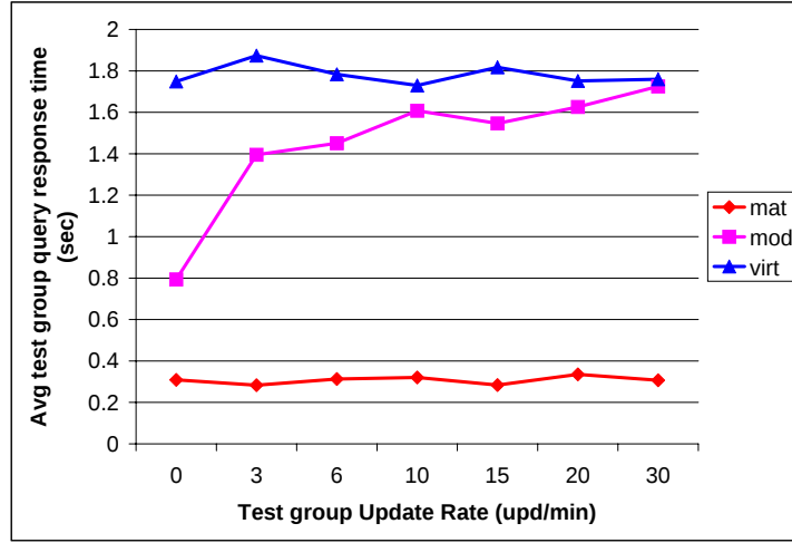
Figure 2: Test group avg query response time
