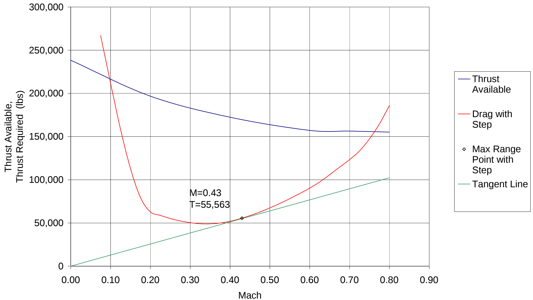
Figure 30. Base Case – 1.0 M lb. Seaplane thrust available, thrust required vs. velocity and max range velocity at sea level
