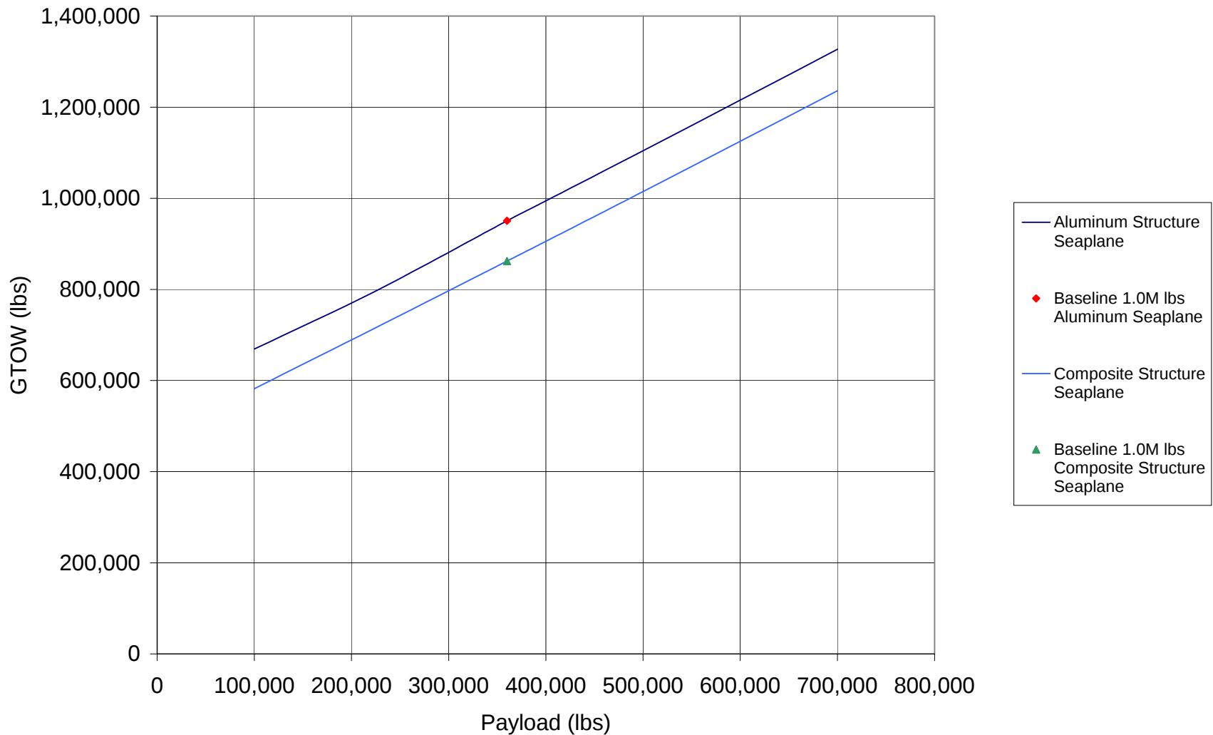
Figure 83. 1.0 M lb. Seaplane with an all aluminum and all composite structure: Payload vs. GTOW
