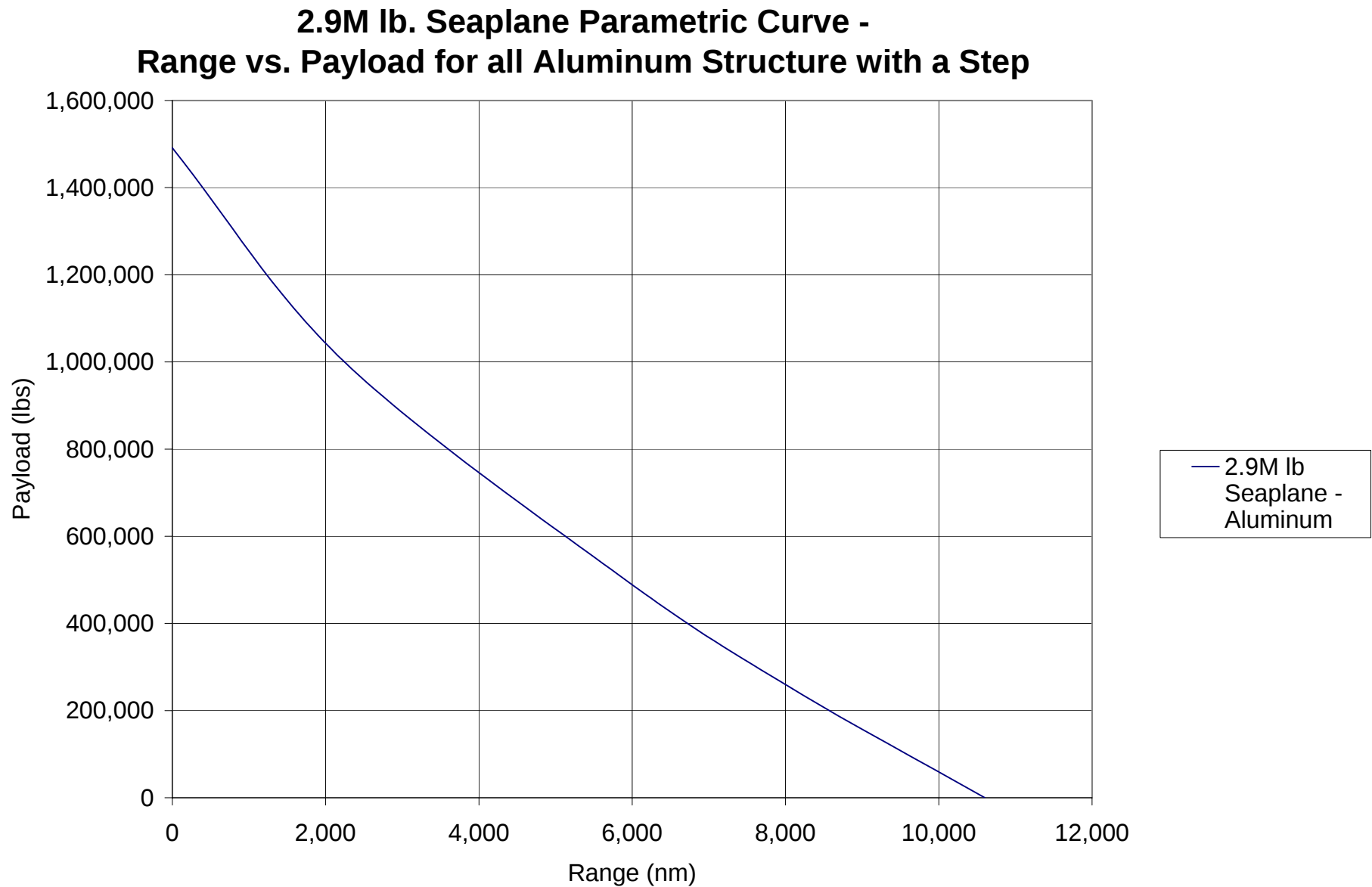
Figure 43. Base Case – 2.9 M lb. Seaplane range vs. payload
