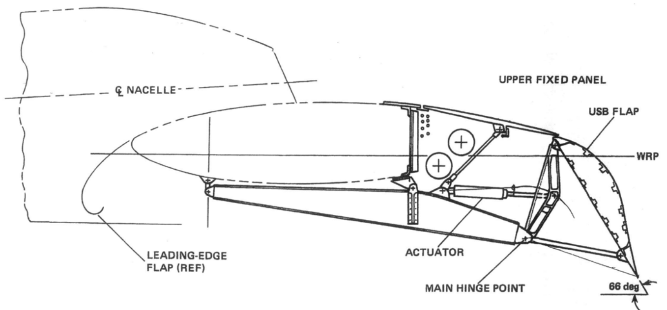
Figure 85. QSRA double slotted flaps.
