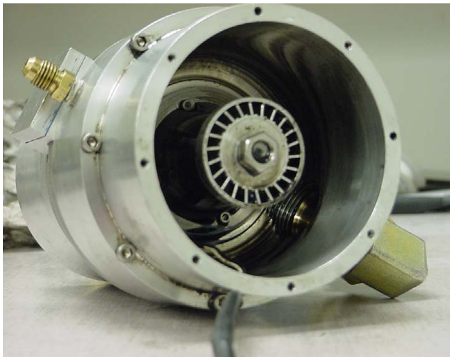
Figure 23: Machined Prototype
