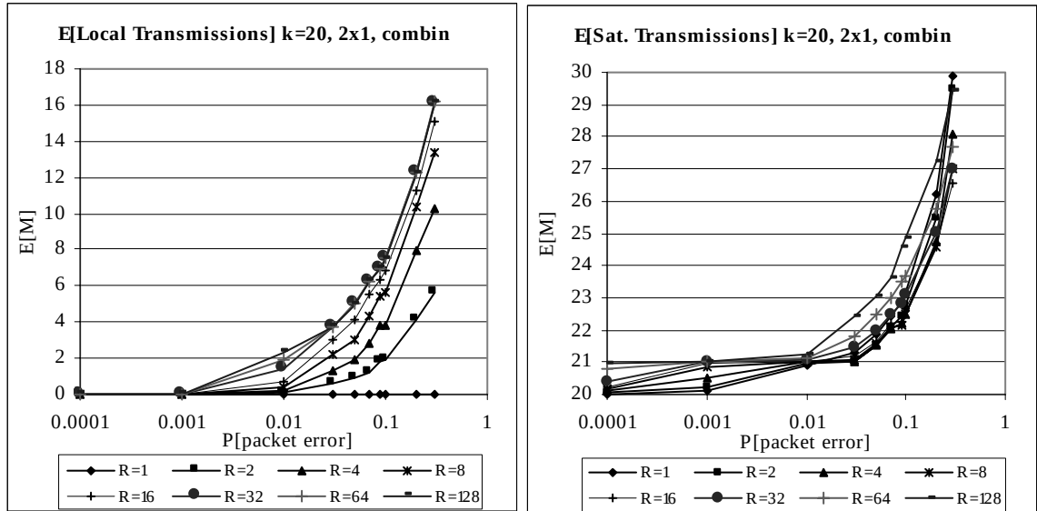
Figure 5.19: Local E[M] & Satellite E[M] k=20, 2x1, combination
