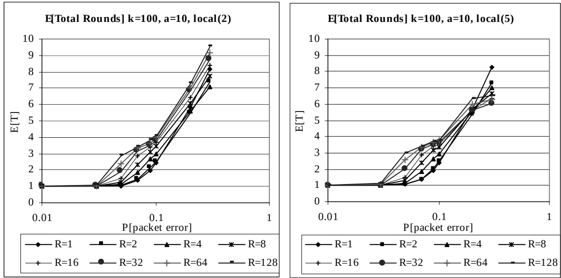
Figure 5.13: E[\text{Total Rounds}] k=100 , a=10 for local(2) and local(5)
