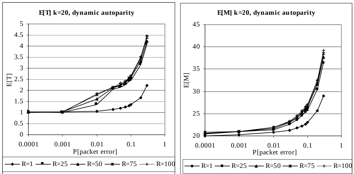
Figure 4.29: E[T] & E[M] for k=20 , dynamic autparity
