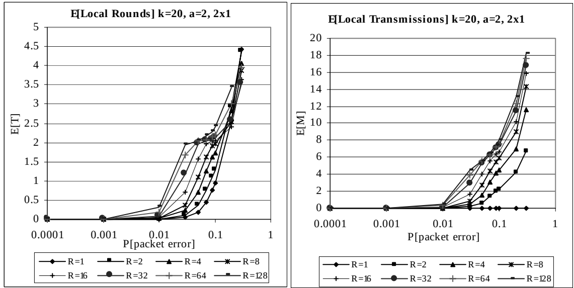
Figure 5.15: E[Local Rounds] & E[Total Rounds] k=20 , a=2 , local(5), 2 \times 1
