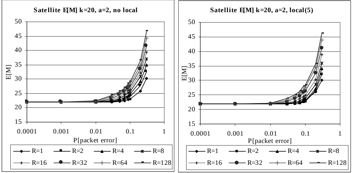
Figure 5.10: Satellite E[M] k=20, a=2 for no local & local(5)
