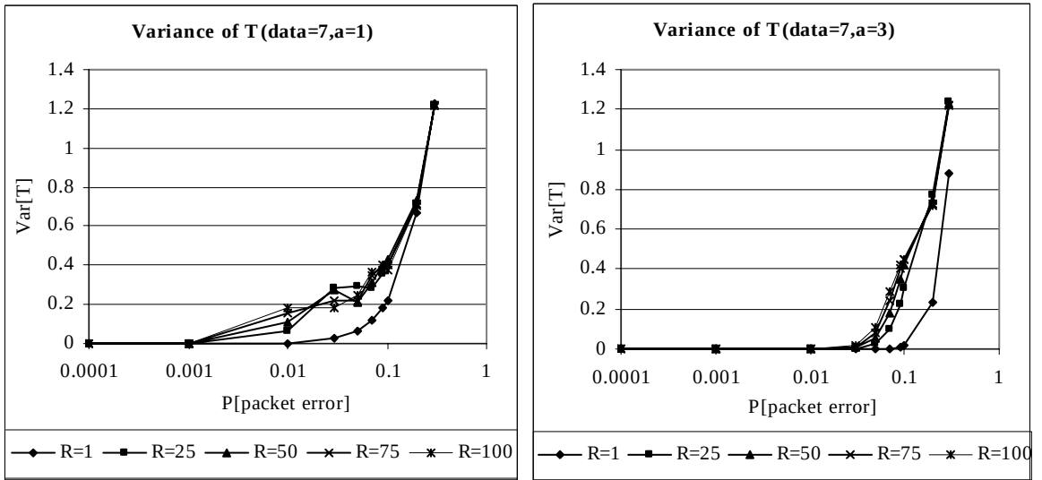
Figure 4.4: \text{Var}[T] versus packet loss probability
