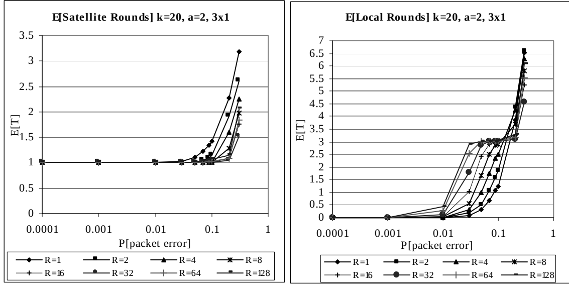
Figure 5.16: E[\text{Satellite Rounds}] & E[\text{Local Rounds}] k=20, a=2, \text{local}(5), 3 \times 1
