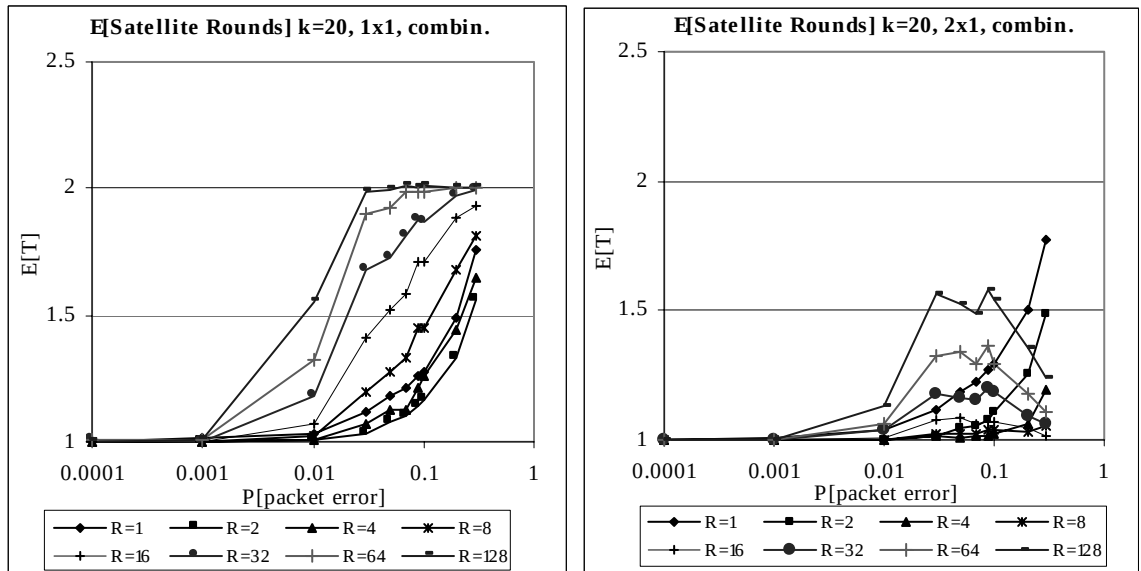
Figure 5.17: E[\text{Satellite Rounds}] k=20 , combination, a=2 , 1 \times 1 and 2 \times 1
