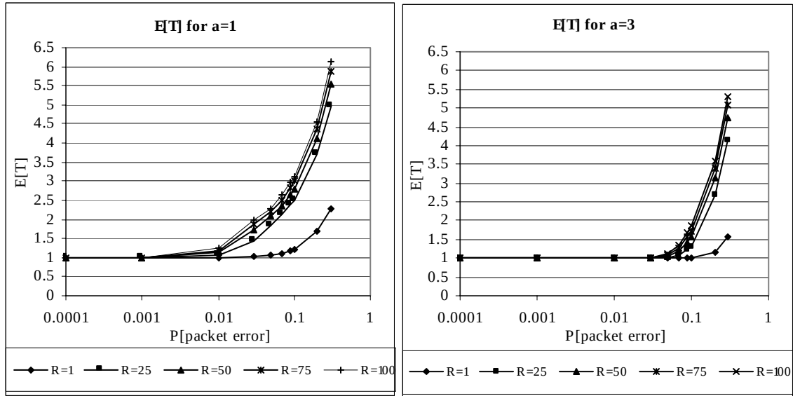
Figure 4.2 E[T] with a=1 & a=3
