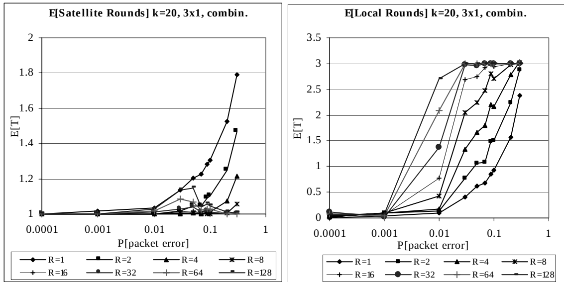
Figure 5.18: E[\text{Satellite Rounds}] & E[\text{Local Rounds}] k=20, combination, 3x1
