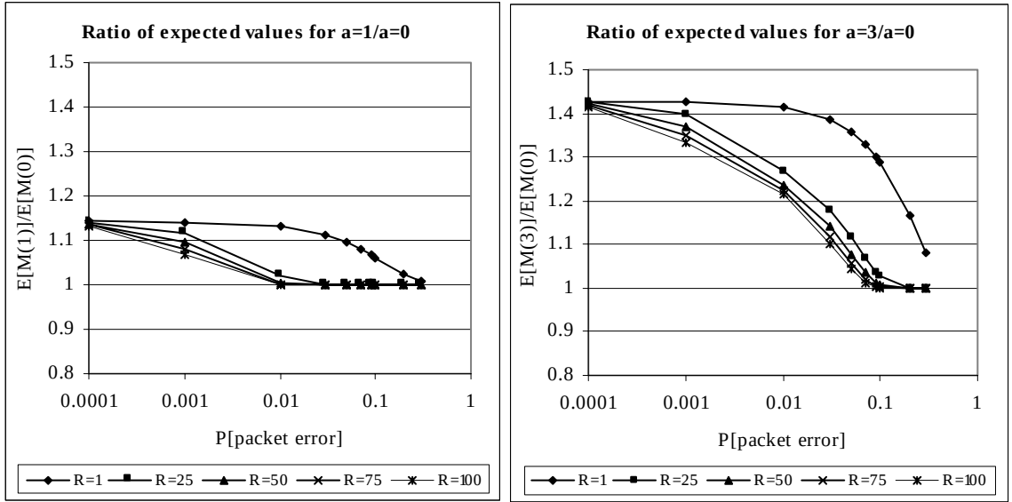
Figure 4.6 Expected value ratios ( a=1/a=0 ) & ( a=3/a=0 )
