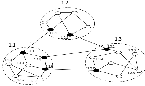
Figure 1: Network with three peer groups – Layer One
