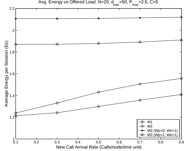
Figure 6: Average energy per session versus per node arrival rate for N = 20 , d_{max} = 50
