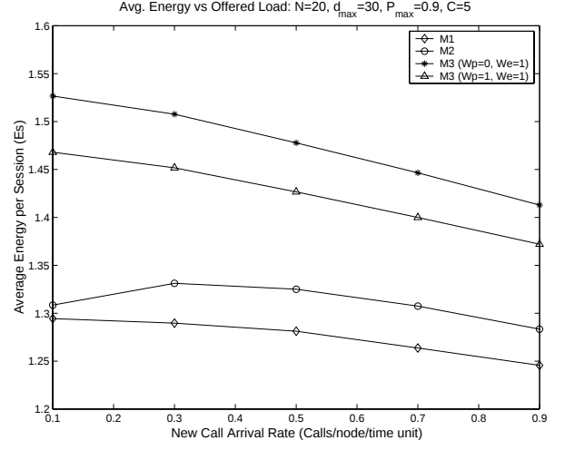
Figure 5: Average energy per session versus per node arrival rate for N = 20 , d_{max} = 30
