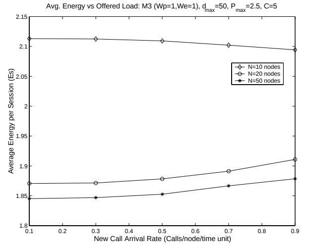
Figure 10: Energy per session vs arrival rate for variable network sizes, M3 and d_{max} = 50
