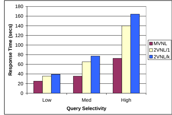
Figure 10: Static queries
