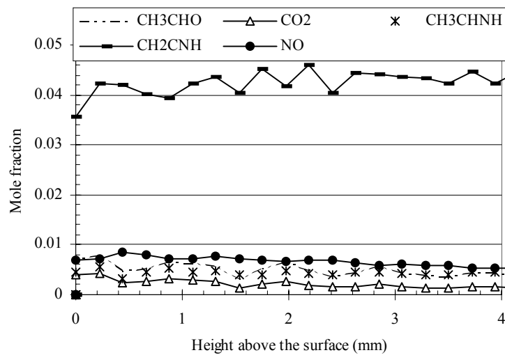
Species profiles and element balance for BAMO/AMMO at 400 \text{ W/cm}^2
