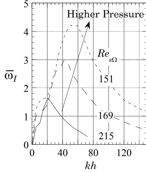
Figure 5. Growth rate of the disturbances for varying chamber pressure ( x/L = 0.5 , \gamma = 1.2148 , Ms = 0.00157 , \Pi = 0.03 )
