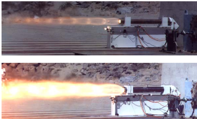
Figure 13. Comparison of Motors No. 7 and 9
