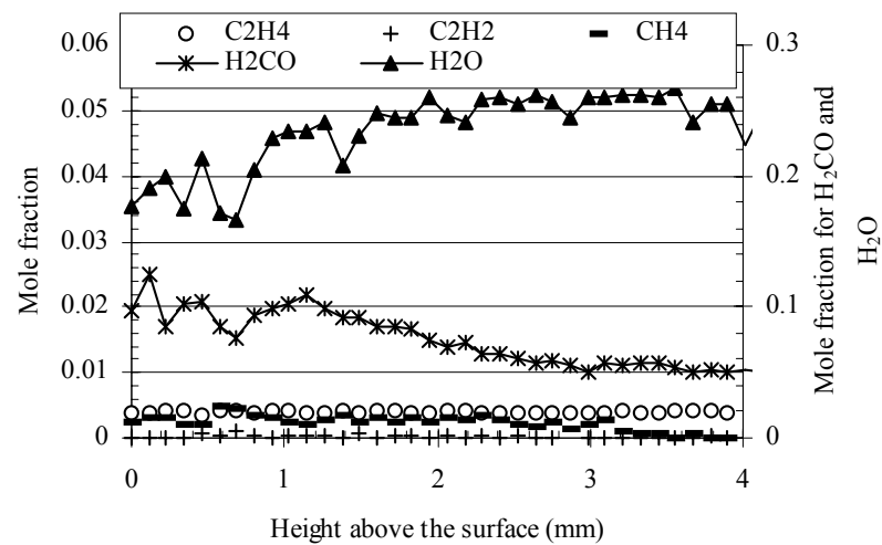
Species and element fraction profiles for deflagration of RDX/BAMO pseudo-propellants at heat flux of 100 \text{ W/cm}^2 in argon at 1 atmosphere.
