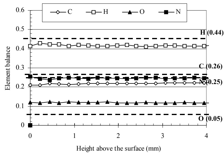
Species profiles and element balance for BAMO/AMMO at 400 \text{ W/cm}^2
