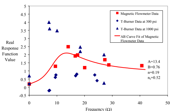
Fig. 6. Propellant 1a response functions comparing NAWC T-burner data and magnetic flowmeter data.
