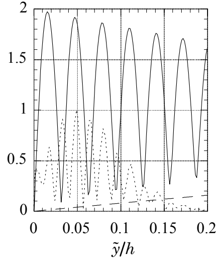
Figure 3. Amplitude of the mean flow, the oscillatory velocity, and disturbance velocity in planar geometry at the condition of NAWC motor #2 pulse 2 ( x/L = 0.5 ). Solid line: oscillatory component. Long-dashed line: mean velocity. Short-dashed line: disturbance velocity
