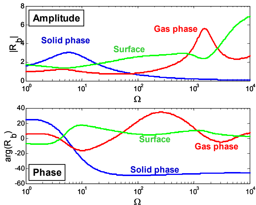
Figure 7. The Combustion Response Function Represented as Magnitudes and Phases of Individual Contributions.
