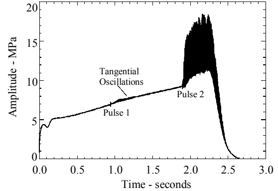
Figure 2. DC Coupled High-Frequency Ballistic Pressure Trace of Motor No. 4
