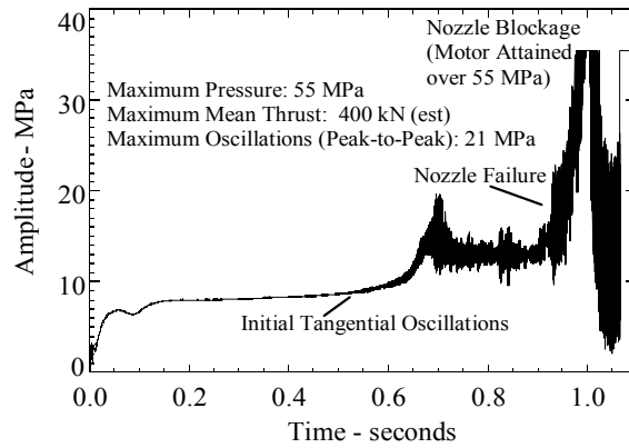
Figure 5. DC Coupled Ballistic Pressure of Motor No. 5
