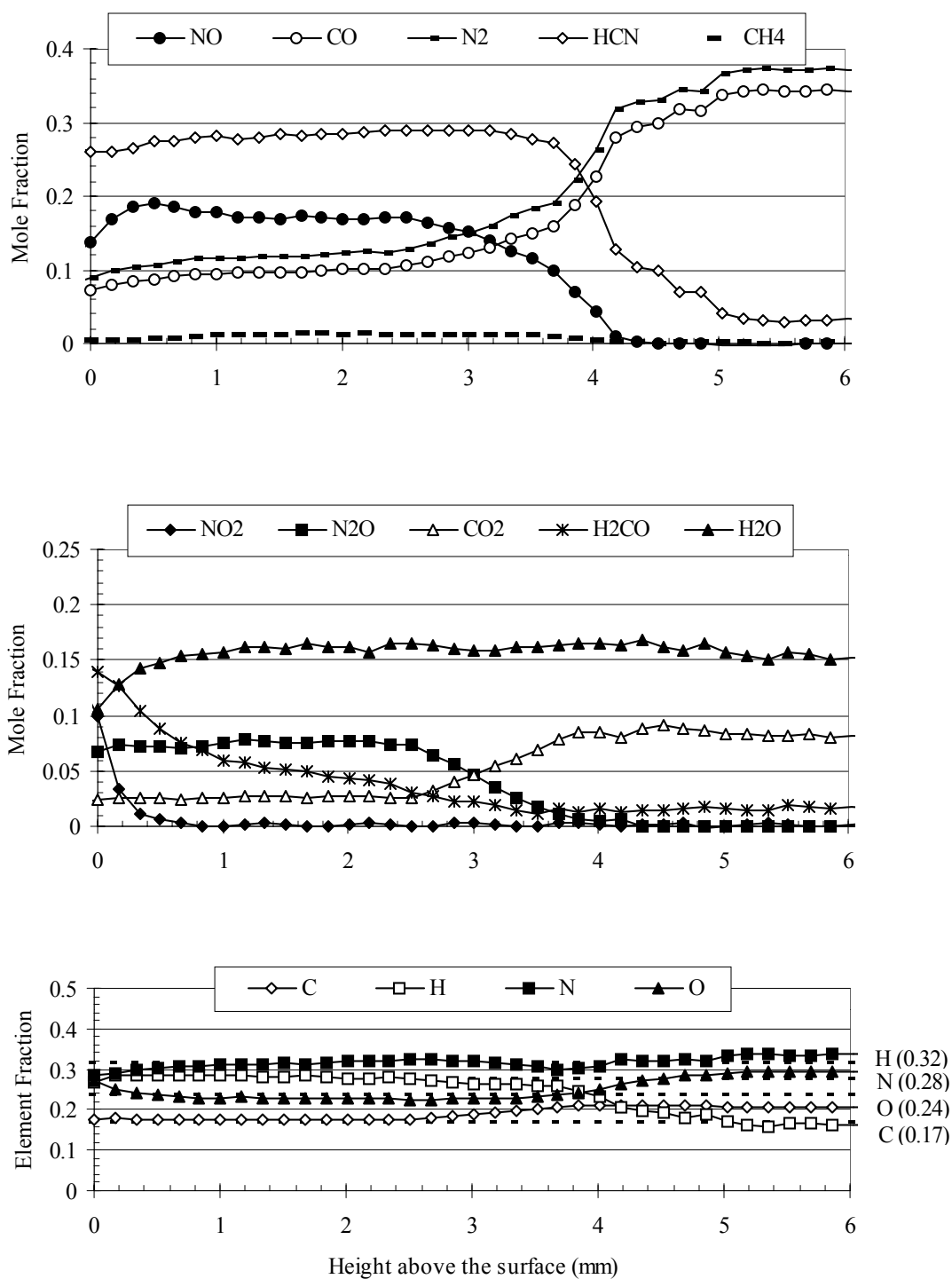
Species and element fraction profiles for deflagration of HMX/GAP pseudo-propellants at heat flux of 100 W/cm 2 in argon at 1 atmosphere.
