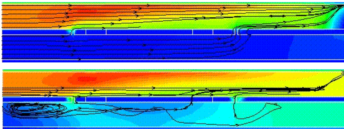
Figure 19: Comparison of flow streamlines and steady-state silane mass fraction contours for hydrogen purge flow rates of 7 slm (top) and 2 slm (bottom). The higher purge flow rate results in zero silane concentration in the lower chamber section, no back-side deposition, and regular flow from inlets to outlet. The lower purge flow rate is ineffective, producing non-zero silane concentration in the lower chamber section and some back-side deposition.
