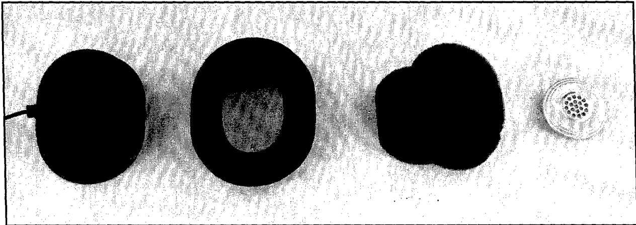
Figure 3. Earcup, earcup seal, insert foam, and speaker (earphone) used in the Gentex HGU-56/P Aircrew Integrated Helmet System.
