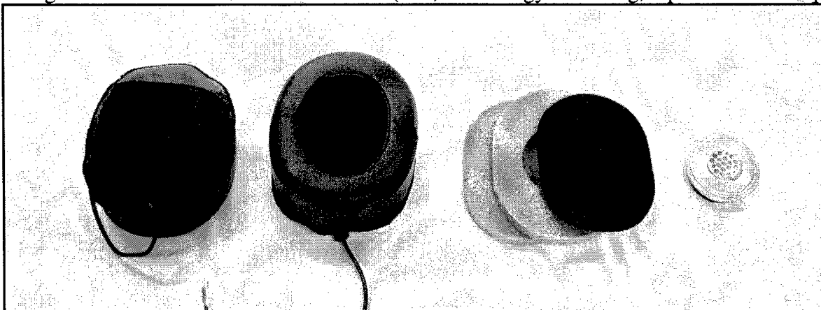
Figure 4. Gentex HGU-56/P Aircrew Integrated Helmet System earcup configuration displayed with the Oregon Aero earcup replacement products evaluated in this study. (a) Oregon Aero HushKit™, (b) Oregon Aero SoftSeal™ with Oregon Aero HushKit™, (c) Oregon Aero SoftSeal/HushKit Combo™
