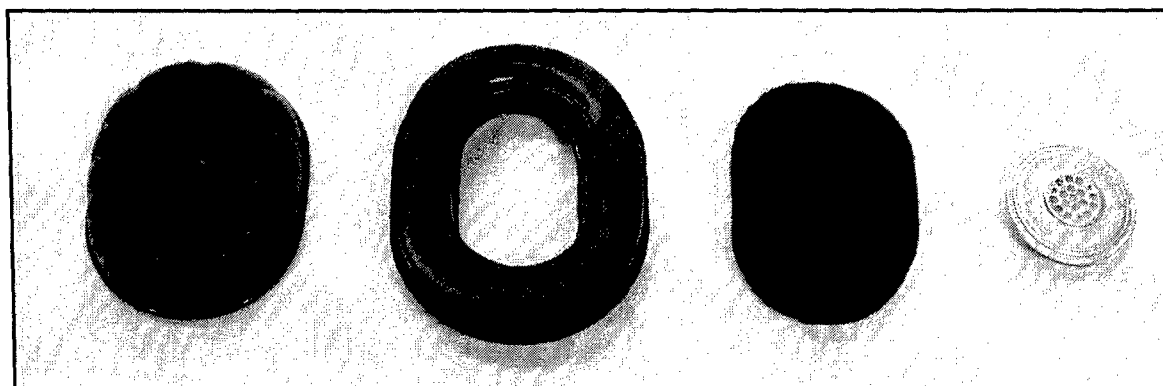
Figure 5. Earcup, earcup seal, insert foam, and speaker (earphone) found in the Gentex HGU-84/P Rotary-Wing Helmet System.
