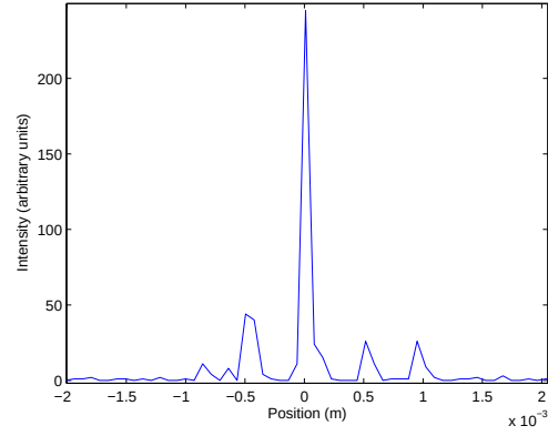
Figure 5.6: Cross-section of the far-field intensity image of the 1.064 \mu\text{m} light through device one at zero bias.
