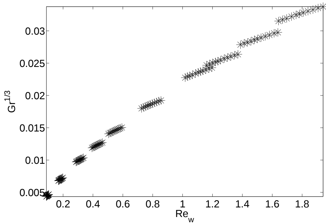
Figure 3.6: Gr^{\frac{1}{3}} vs. Re_w for all contraction Reynolds numbers
