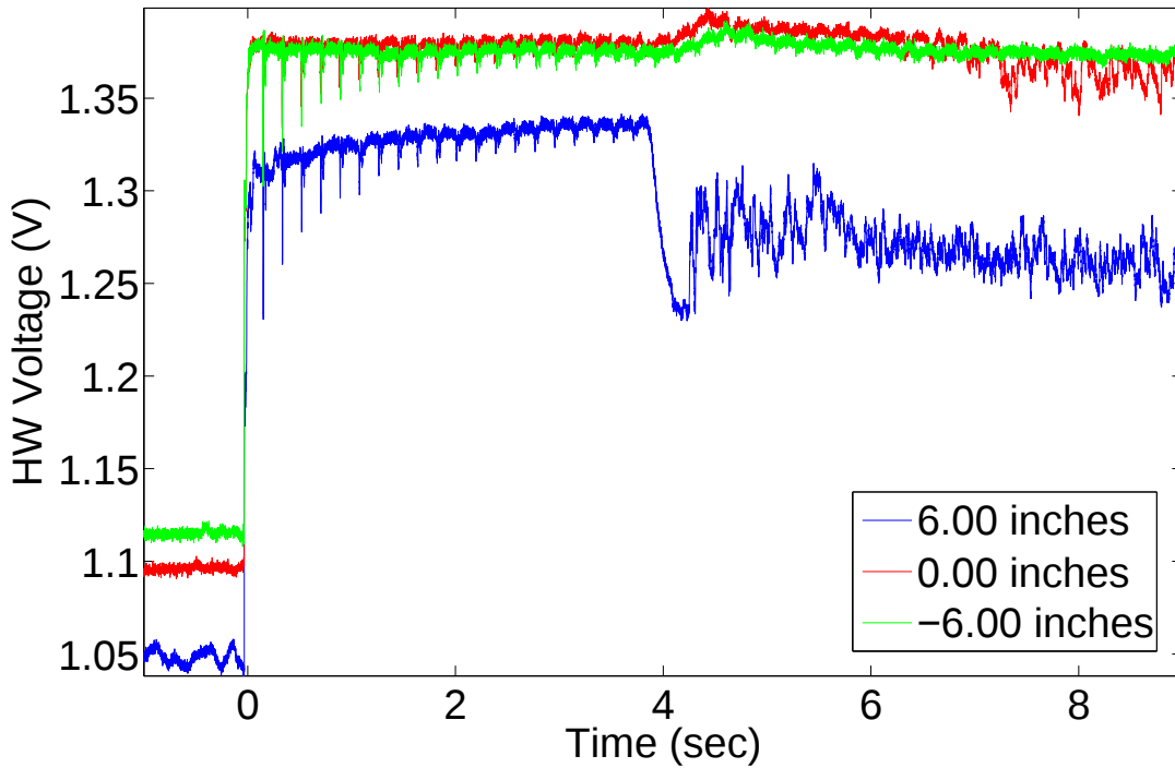
Figure 7.2: Oscilloscope traces at y_c=6.00 , 0.00 and -6.00 inches for 45 psia
