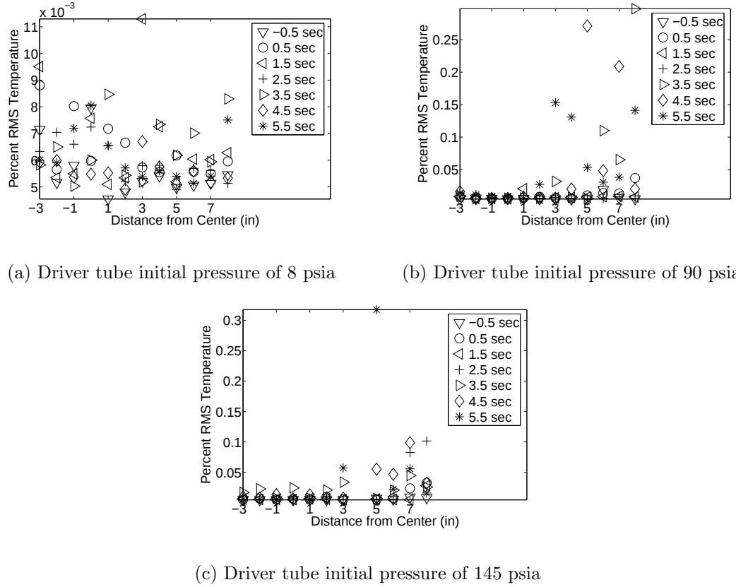
Figure 4.6: RMS temperature for partially heated driver tube at 8, 90, and 145 psia
