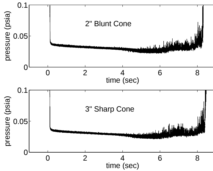
Figure 31: Diffuser static pressure at z=105.0 inches.
