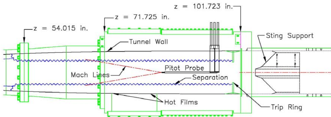
Figure 78: Schematic of the end of the nozzle with 2.5 inch trips.
