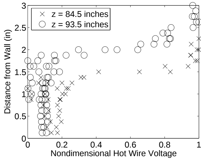
Figure 71: Profiles of separation with hot wire, with an initial driver tube pressure of 8 psia.
