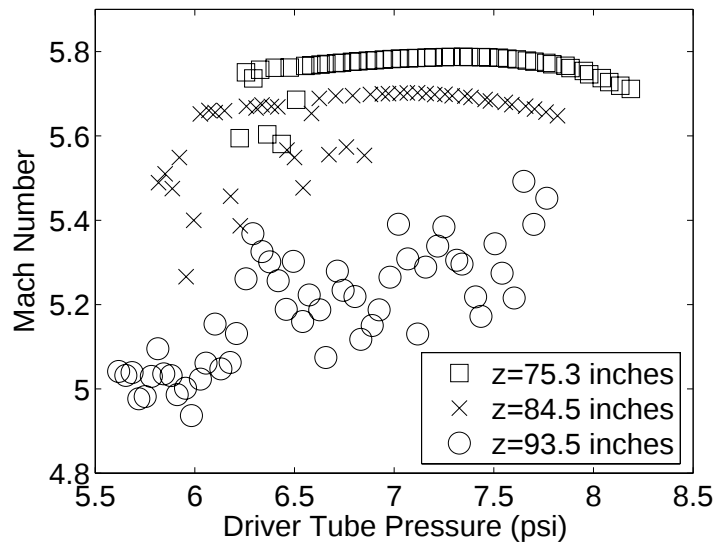
Figure 37: Effect of axial location on Mach number with pressure below 8 psia.
