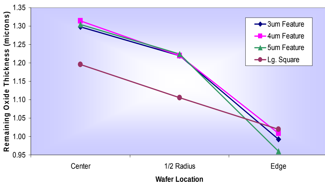
Figure 39. WIWNU measurement for wafers after timed-CMP
