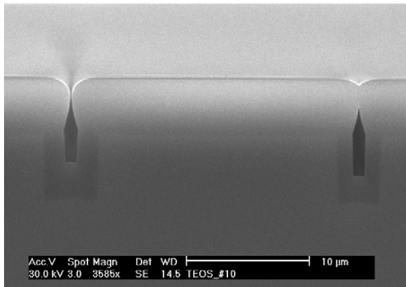
Figure 15. Keyholes in ATP TEOS fill
