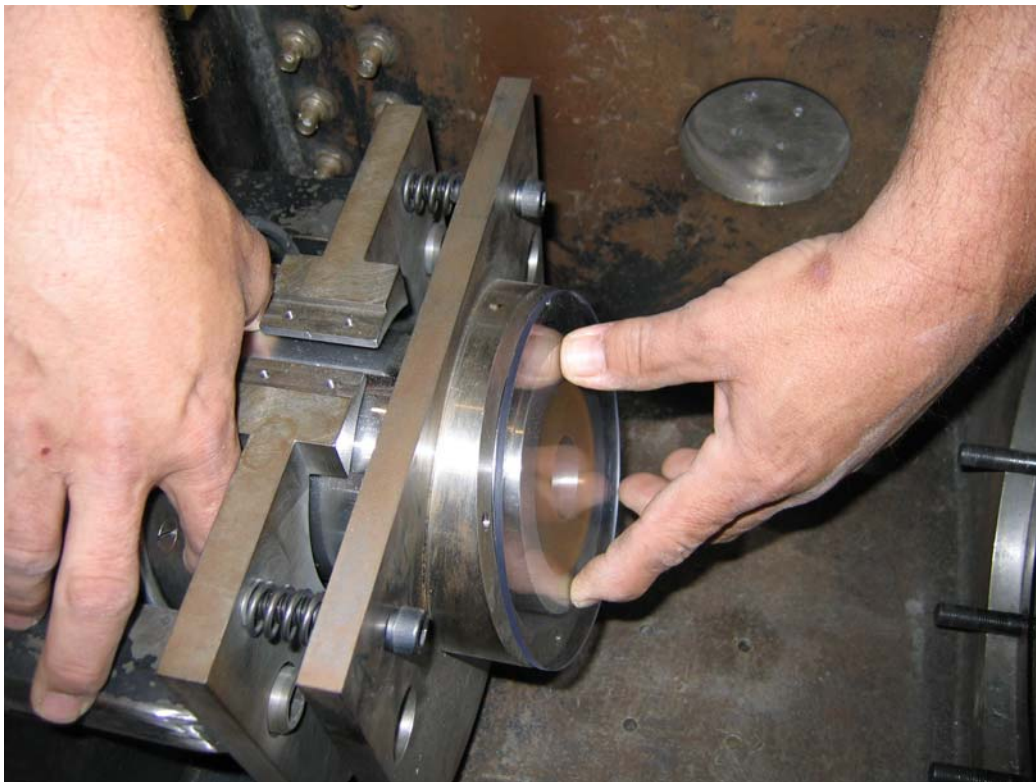
Figure 12. Aligning flyer assembly with 6-in lexan ring.
