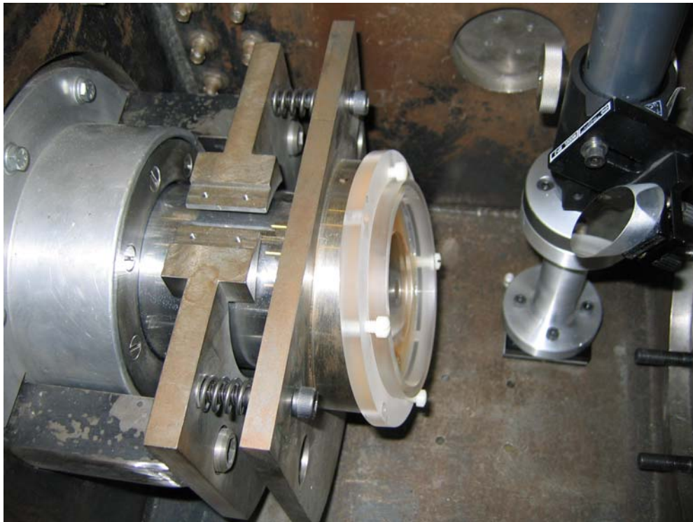
Figure 20. Nylon target mounting screws with plate assemblies.
