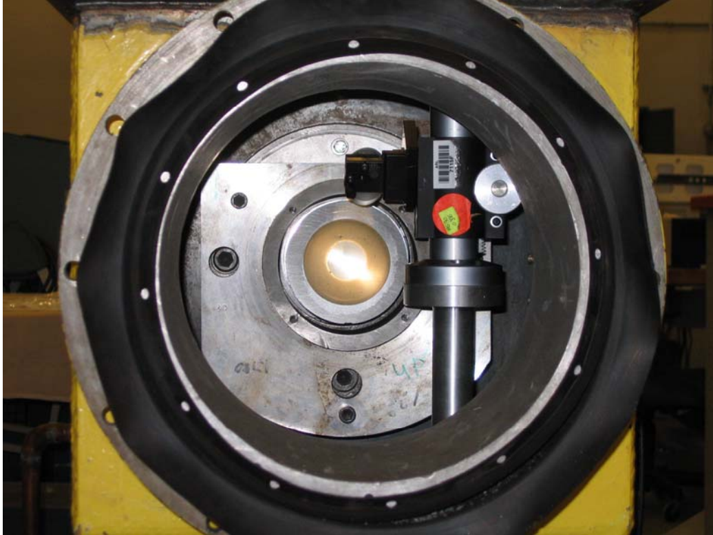
Figure 14. View of optic towers off axis alignment.
