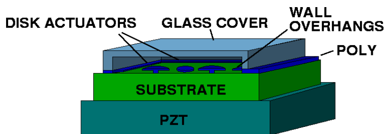
Figure 3.1 Microfluidic Actuator
