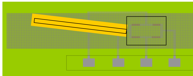
(f) A mold is then patterned over the seed layer such that the cantilever part of the mold lies over the gold sacrificial layer.
