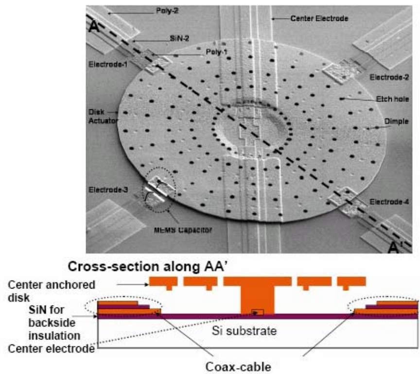
Figure 3.5 SEM of Actuator Structure and Cross Section View
