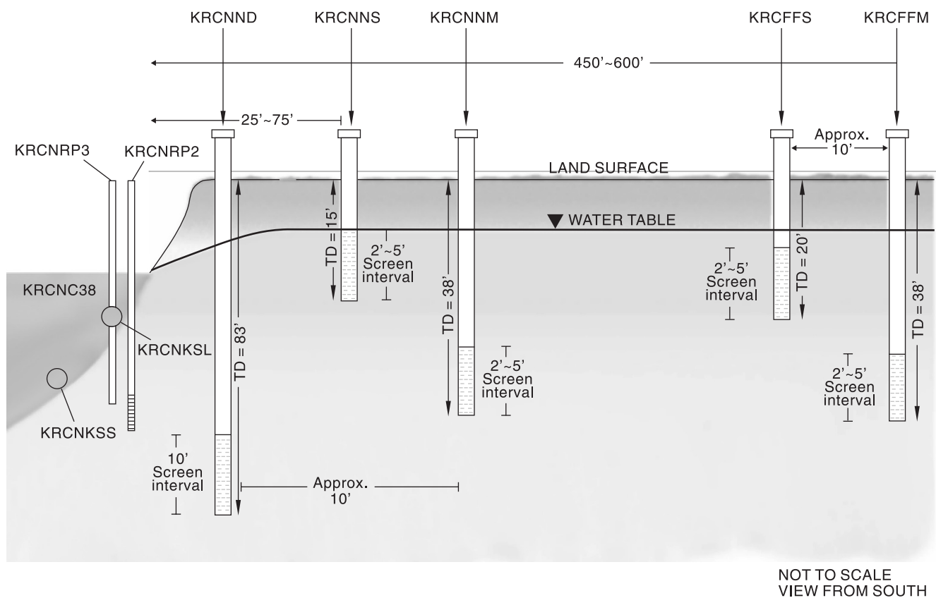
Figure 2. Generalized well layout and construction details for Site C, east bank of C-38 (Pool C).
