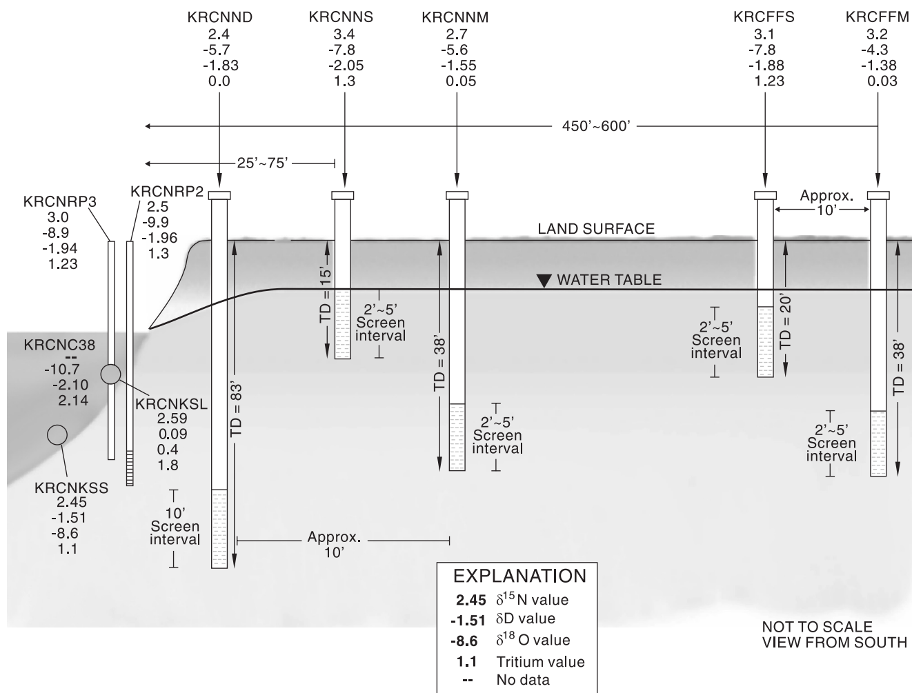
Figure 8. Distribution of tritium and oxygen, hydrogen, and nitrogen isotope data for Site C.
