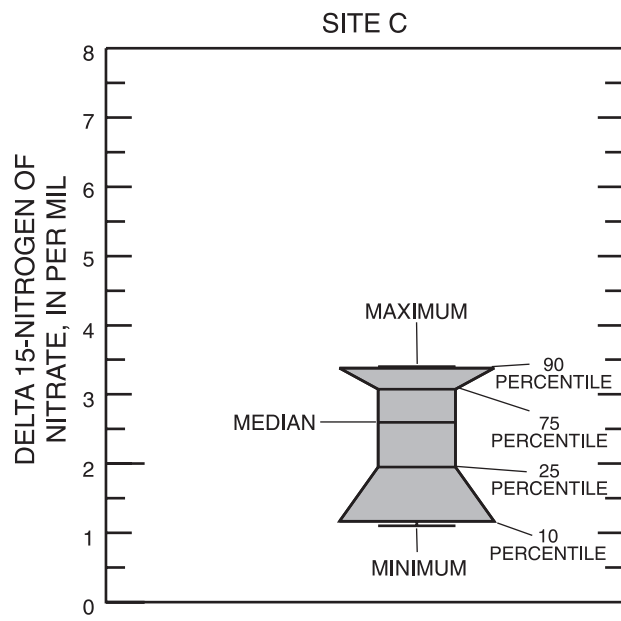
Figure 11. Delta nitrogen-15 data.
