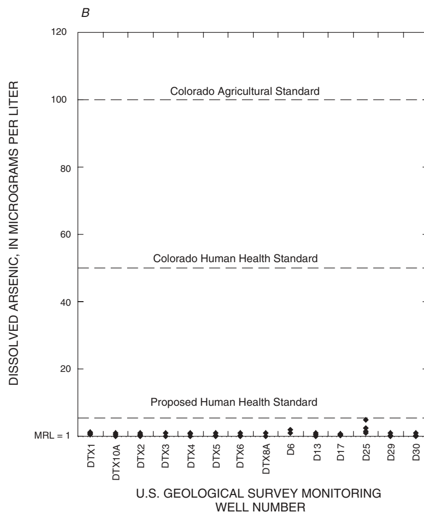
Figure 11. Distribution of ground-water data collected near Deer Trail, Colorado, compared to regulatory standards for selected constituents, 1999—Continued.
