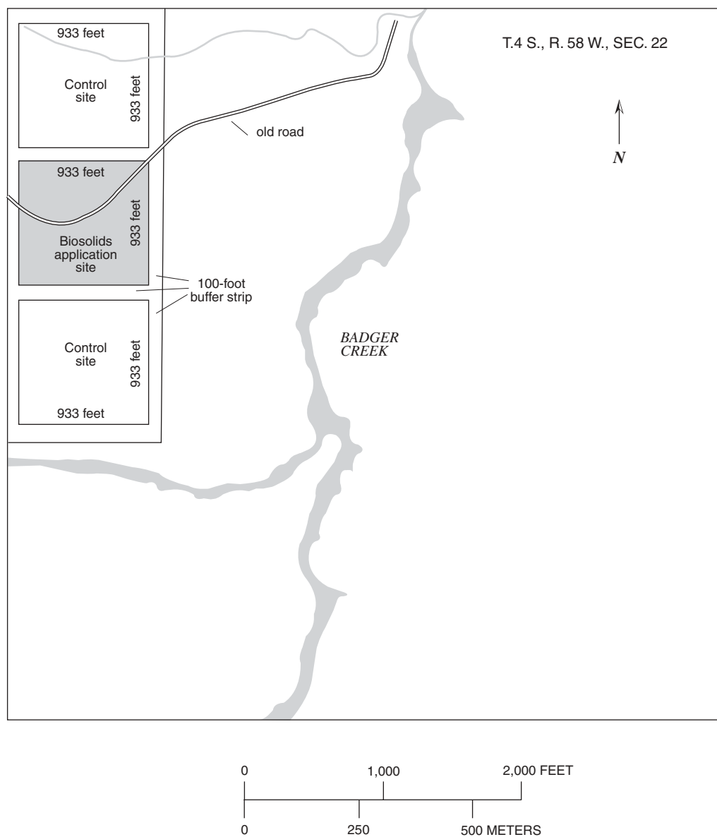
Figure 3. Arapahoe County, Colorado, soil-monitoring site: T. 4 S., R. 58 W., sec. 22 (modified from Metro Wastewater Reclamation District).
