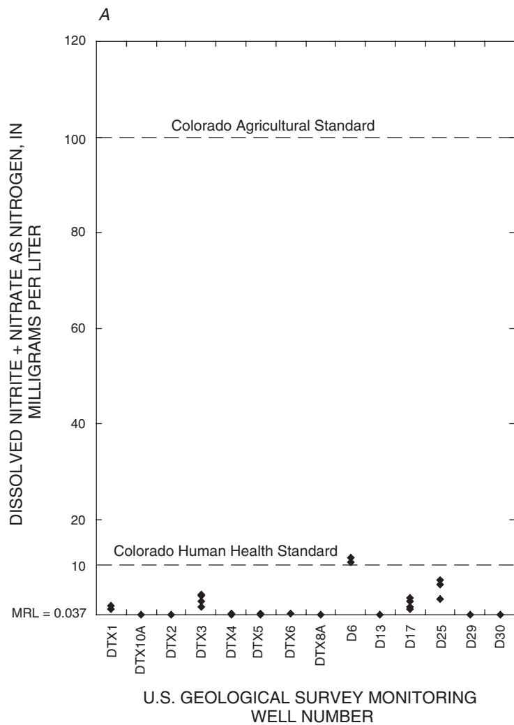
Figure 11. Distribution of ground-water data collected near Deer Trail, Colorado, compared to regulatory standards for selected constituents, 1999.
