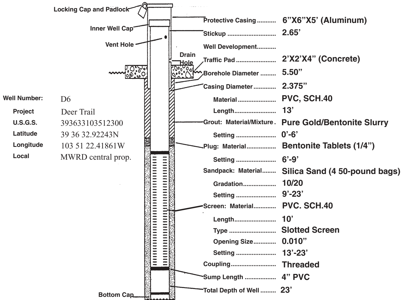
U.S. Geological Survey Well
