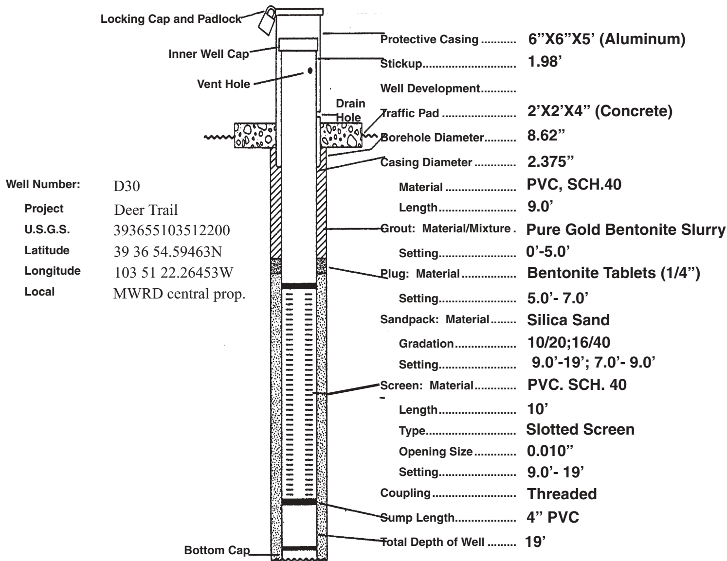
U.S. Geological Survey Well
