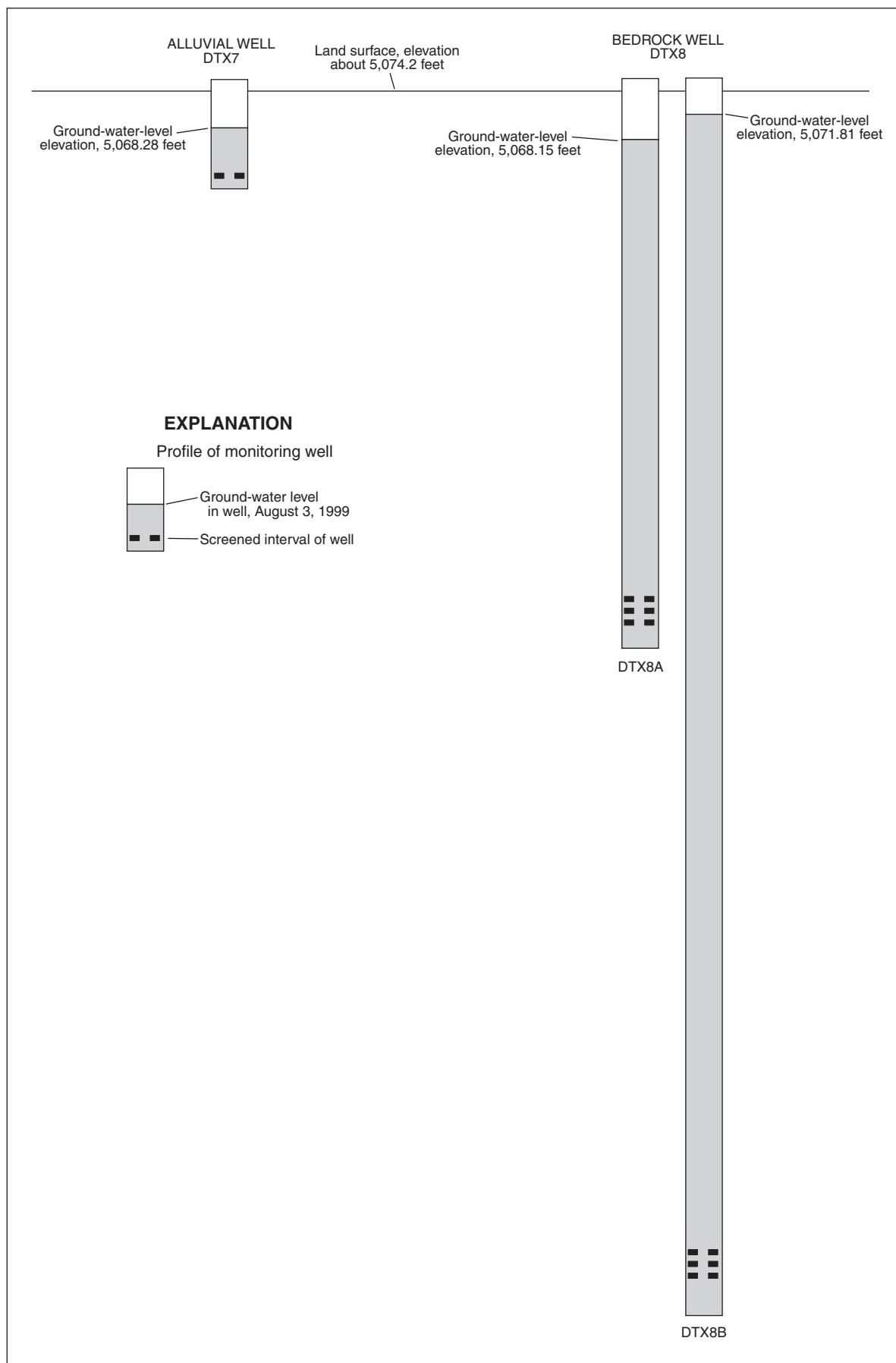
Figure 9. Water levels for the recharge-evaluation site containing well DTX7 and nested well DTX8 (includes DTX8A and DTX8B) near Deer Trail, Colorado, for July, August, and September 1999—Continued.
