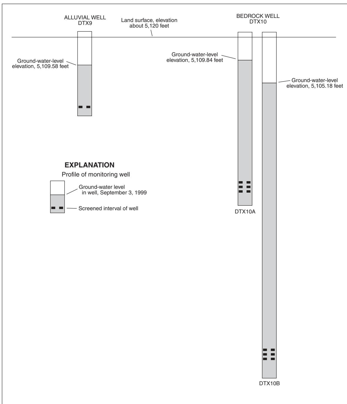
Figure 10. Water levels for the recharge-evaluation site containing well DTX9 and nested well DTX10 (includes DTX10A and DTX10B) near Deer Trail, Colorado, for July, August, and September 1999—Continued.
