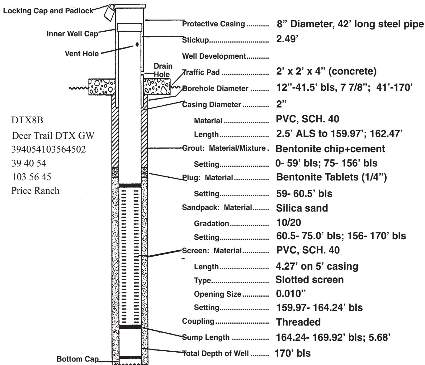
U.S. Geological Survey Well
