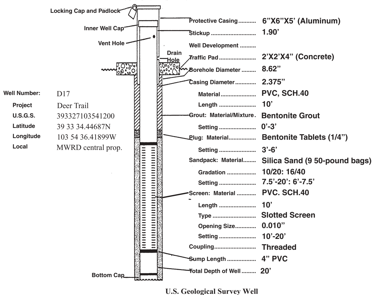
Figure 5. Well-completion information for USGS monitoring wells near Deer Trail, Colorado, 1999 (latitude and longitude are in degrees minutes seconds; PVC, polyvinyl chloride; SCH., schedule; ALS, above land surface; bls, below land surface; prop., property; Na, sodium)—Continued.
