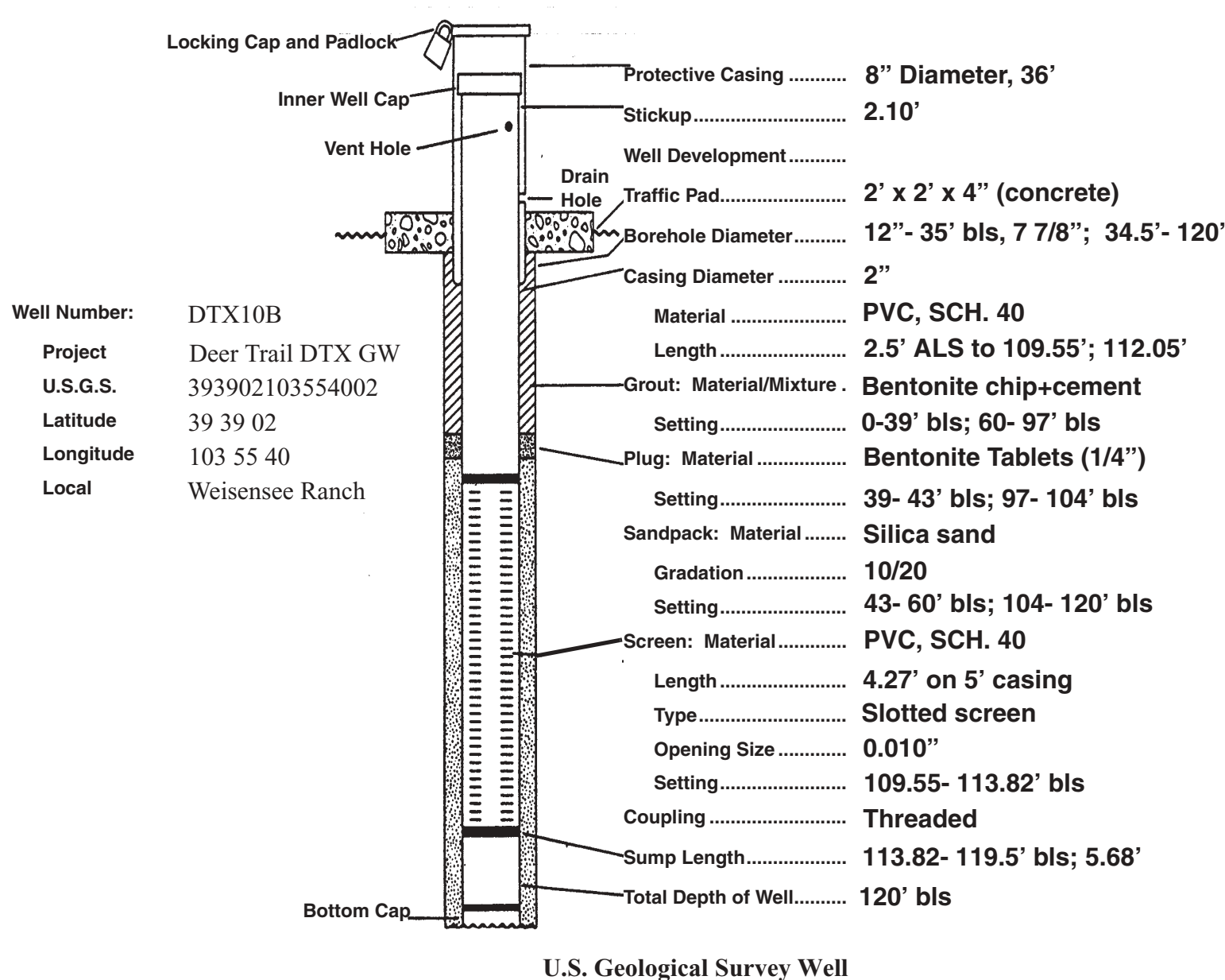
Figure 5. Well-completion information for USGS monitoring wells near Deer Trail, Colorado, 1999 (latitude and longitude are in degrees minutes seconds; PVC, polyvinyl chloride; SCH., schedule; ALS, above land surface; bls, below land surface; prop., property; Na, sodium)—Continued.
