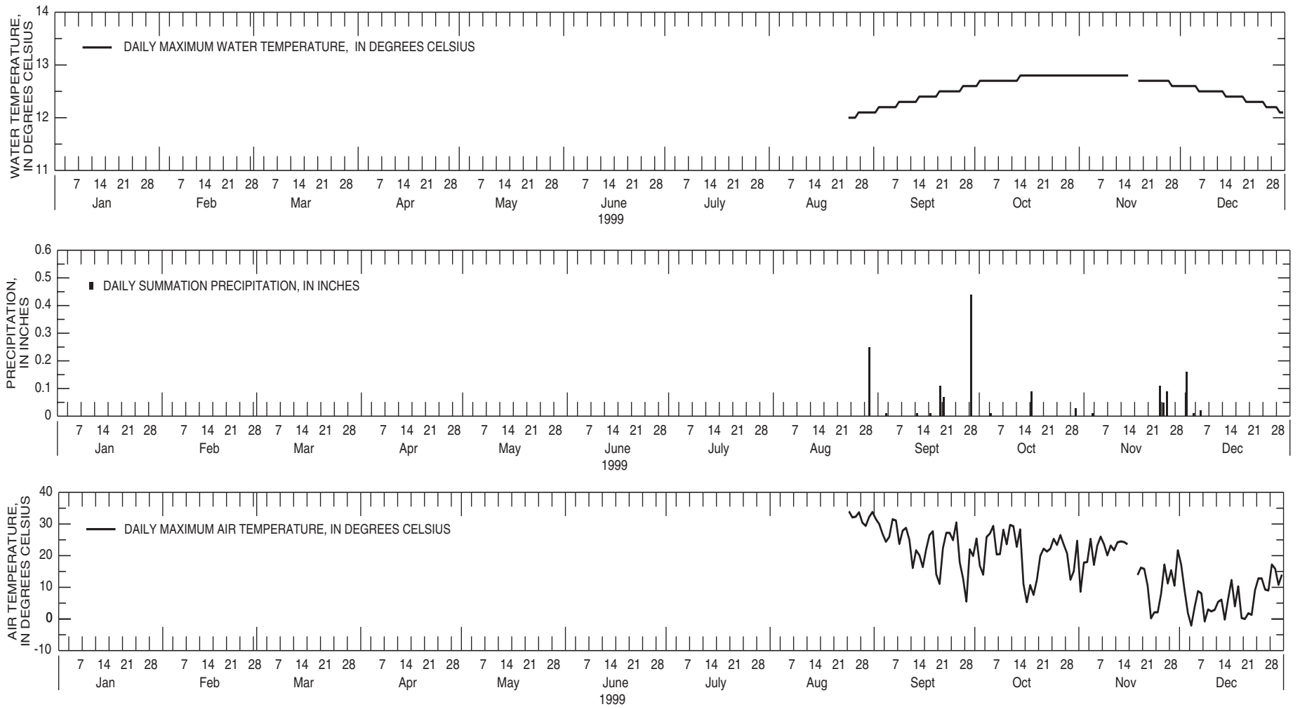
Figure 8. Continuous water-temperature, precipitation, and air-temperature data for well DTX5 near Deer Trail, Colorado, 1999. No water-level data are available. Data collection began in August.
