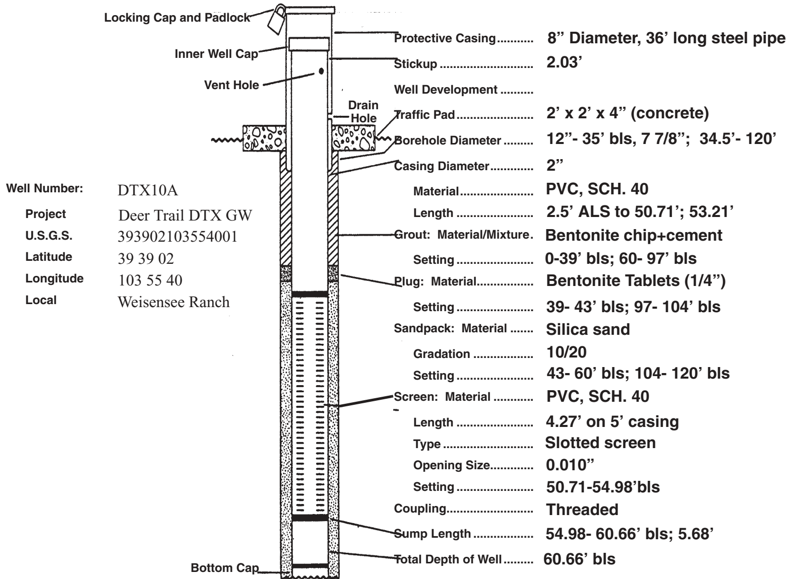
U.S. Geological Survey Well
