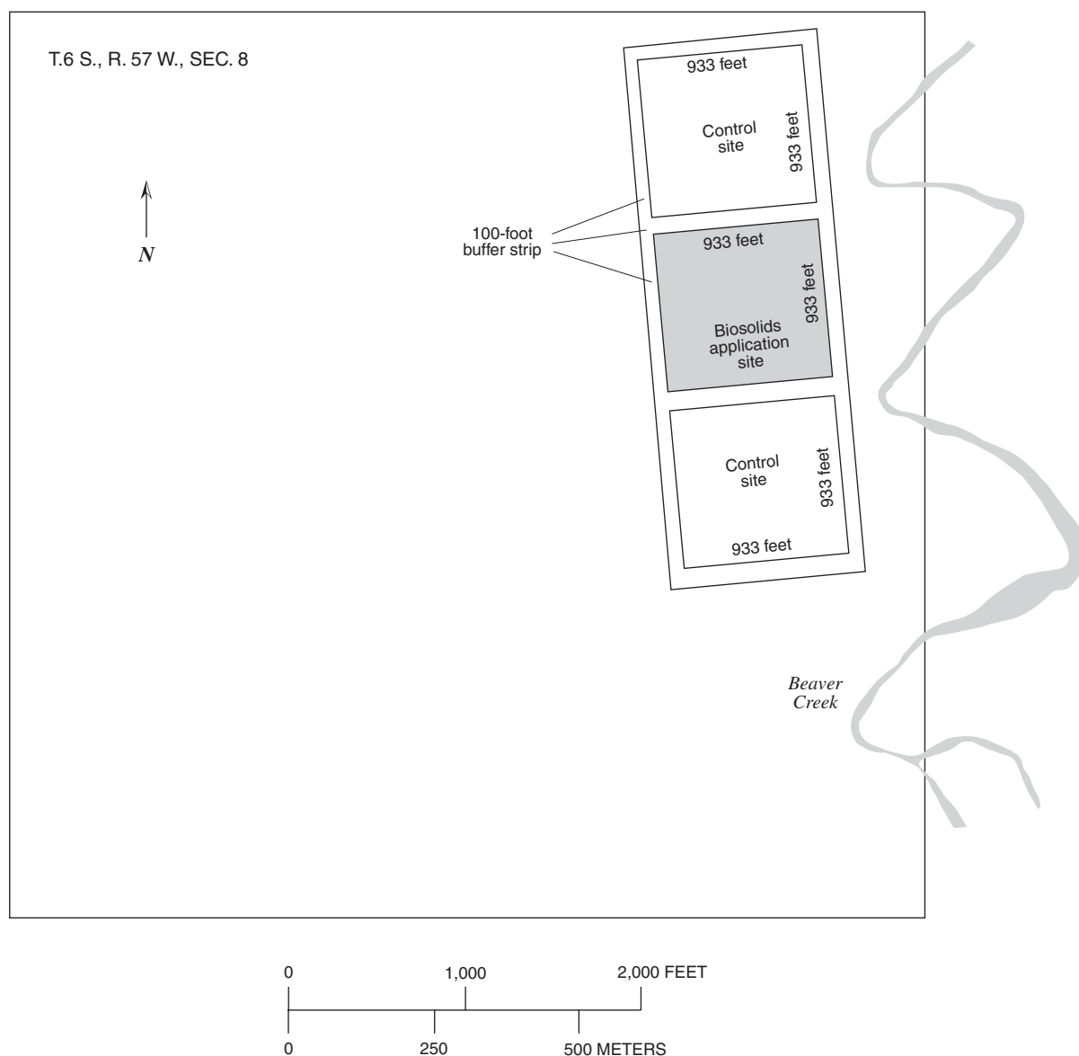
Figure 4. Elbert County, Colorado, soil-monitoring site: T. 6 S., R. 57 W., sec. 8 (modified from Metro Wastewater Reclamation District).
