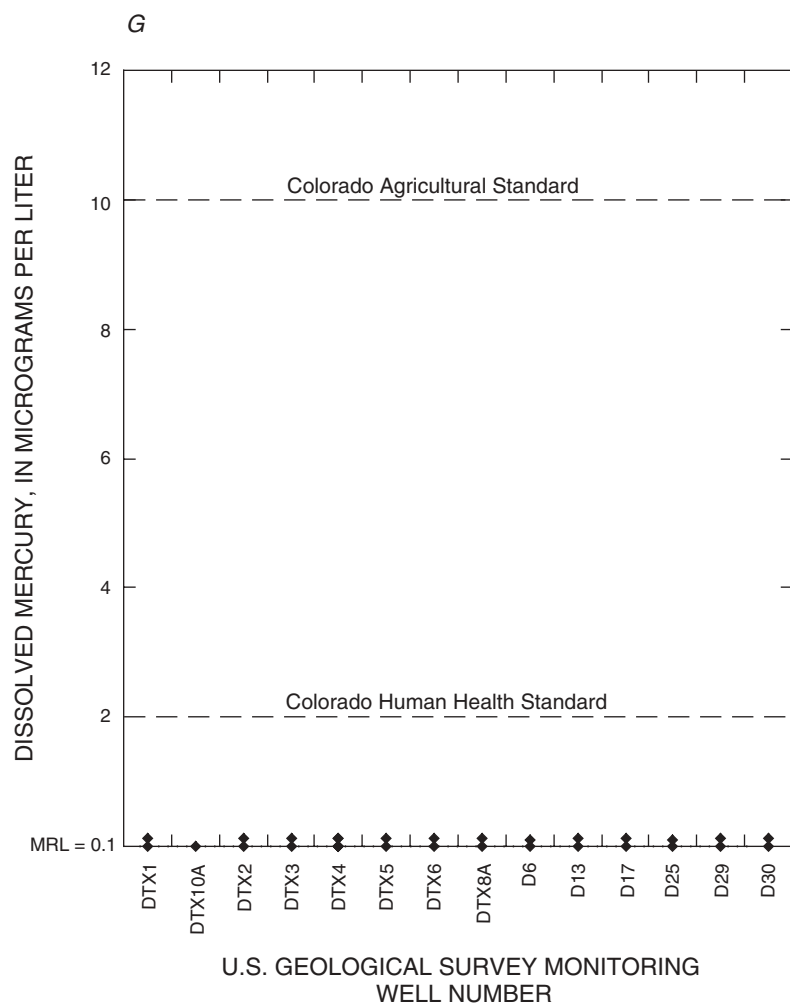
Figure 11. Distribution of ground-water data collected near Deer Trail, Colorado, compared to regulatory standards for selected constituents, 1999—Continued.
