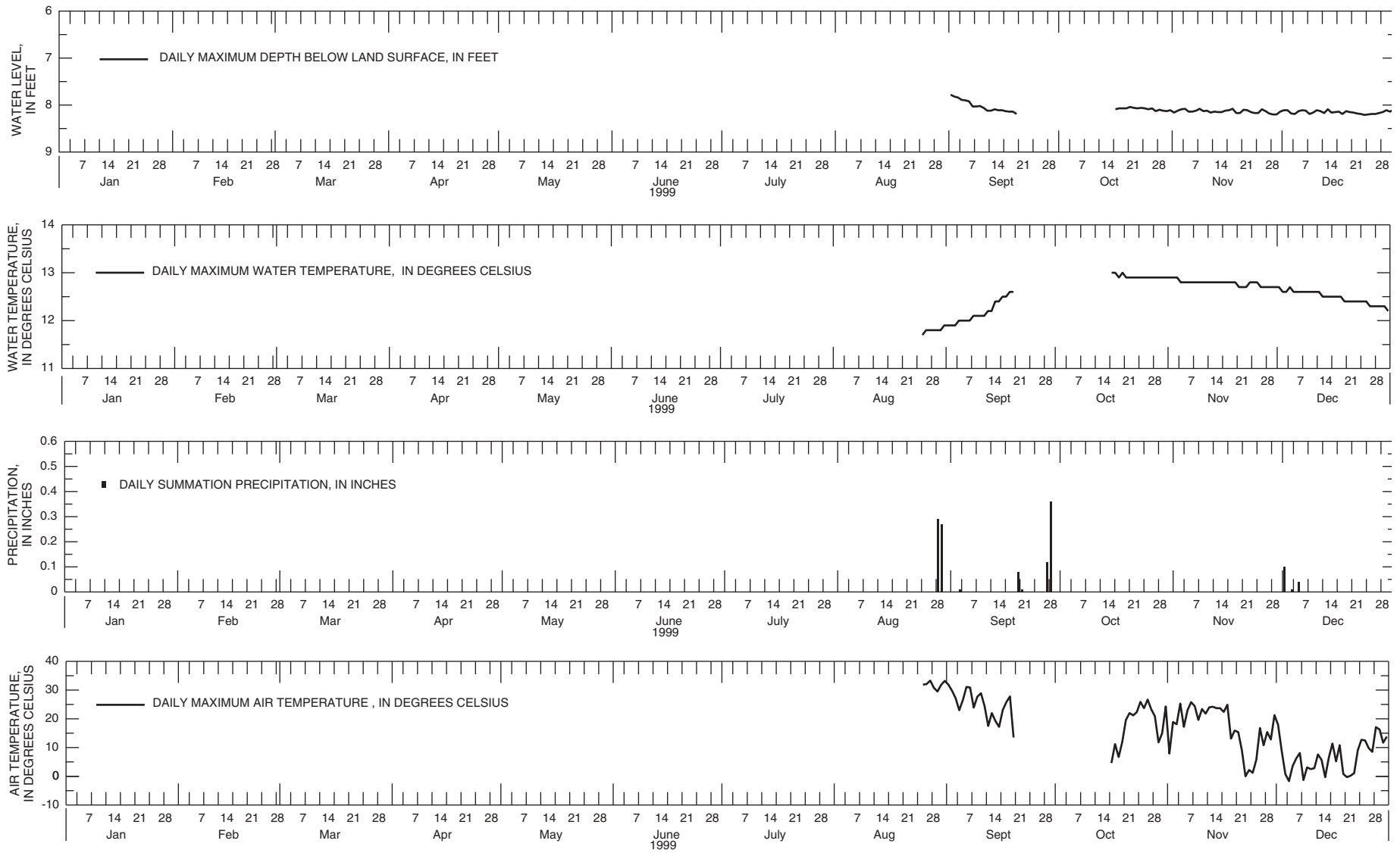
Figure 6. Continuous water-level, water-temperature, precipitation, and air-temperature data for well D25 near Deer Trail, Colorado, 1999. Data collection began in August.
