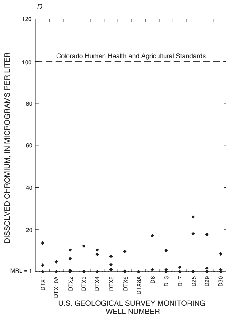
Figure 11. Distribution of ground-water data collected near Deer Trail, Colorado, compared to regulatory standards for selected constituents, 1999—Continued.
