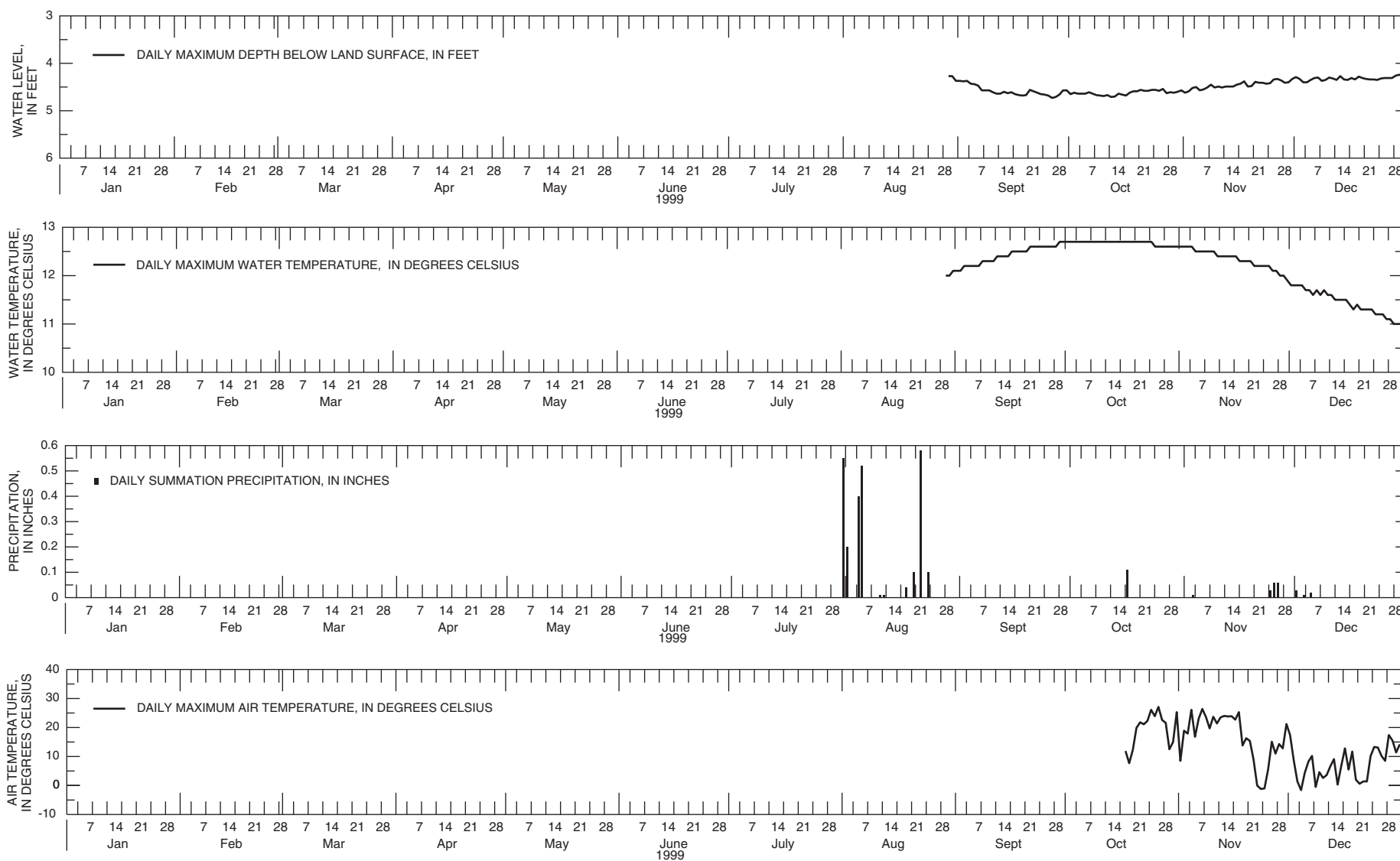
Figure 7. Continuous water-level, water-temperature, precipitation, and air-temperature data for well DTX2 near Deer Trail, Colorado, 1999. Data collection began August-October.
