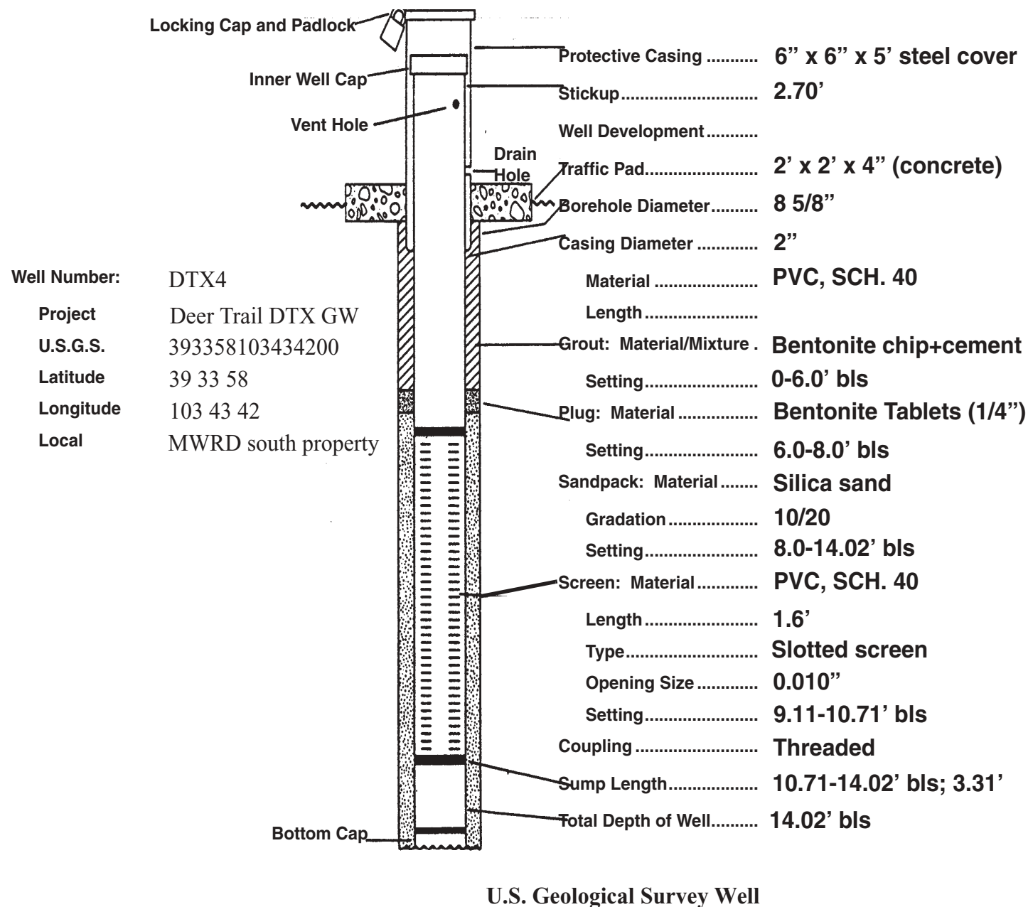
Figure 5. Well-completion information for USGS monitoring wells near Deer Trail, Colorado, 1999 (latitude and longitude are in degrees minutes seconds; PVC, polyvinyl chloride; SCH., schedule; ALS, above land surface; bls, below land surface; prop., property; Na, sodium)—Continued.
