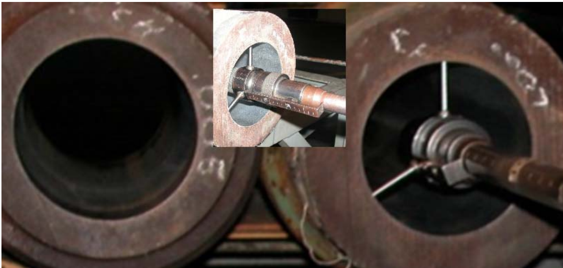
Figure 5. Star-gauging scrap sections of the M256 barrel.
