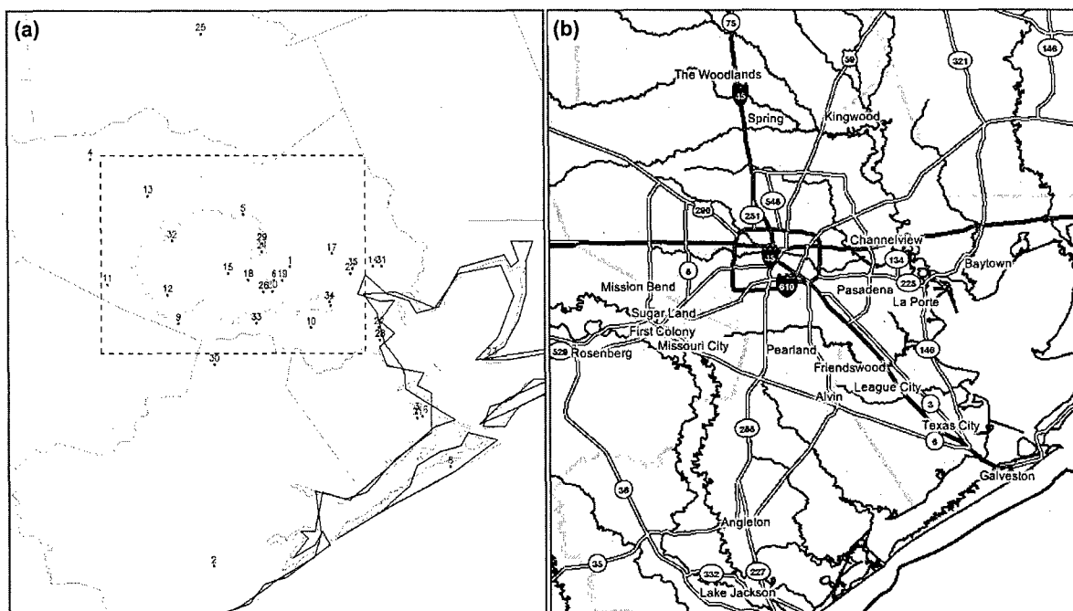
Figure 2. (a) Location of 35 Continuous Ambient Monitoring Stations (CAMS) operated by the Texas Commission on Environmental Quality (TCEQ) providing mean hourly surface measurements of temperature and winds (speed and direction); sites number in blue also provide mean hourly measurements of \text{SO}_2 concentrations. (b) Detailed map of the CAMS analysis area depicting the location of major roadways as well as prominent water features throughout the area.
