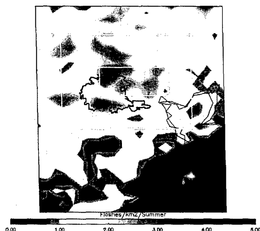
Figure 3. Spatial variations of mean flash density (valid 0900-1859 CST) for 336 non-contiguous days resulting from the application of SE1 and the first half of SE2. Domain and spatial references correspond to zoomed portion of Figure 1.
