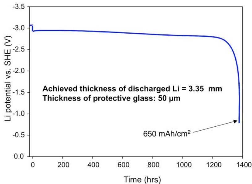
Fig. 1. Discharge of thick protected Li in 4 M NH 4 Cl aqueous electrolyte at 0.5 mA/cm 2 .
