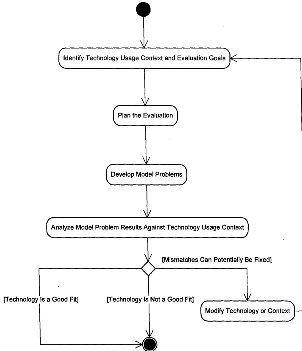
Figure 1: Context-Based Technology Evaluation Method
