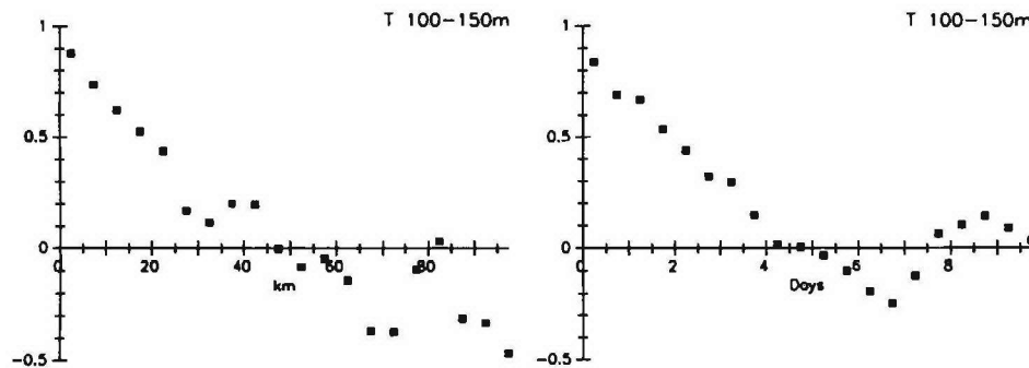
Figure 3. Spatially (left) and temporally (right) lagged correlation of the average temperature between 100 and 150 m depth showing characteristic scales of 2 days and 15 km.
