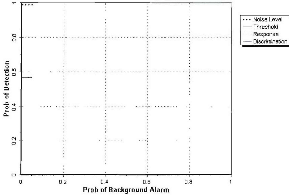
Figure 3. EM61 MKII/man-portable blind grid probability of detection for response and discrimination stages versus their respective probability of background alarm over all ordnance categories combined.
