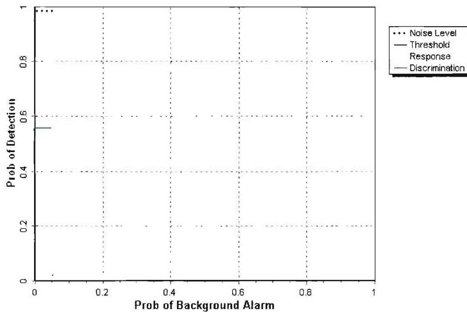
Figure 5. EM61 MKII/man-portable blind grid probability of detection for response and discrimination stages versus their respective probabilities of background alarm for all ordnance larger than 20 mm.
