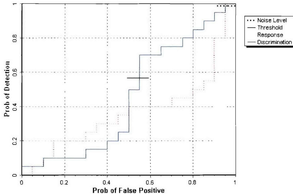
Figure 2. EM61 MKII/man-portable blind grid probability of detection for response and discrimination stages versus their respective probability of false positive over all ordnance categories combined.
