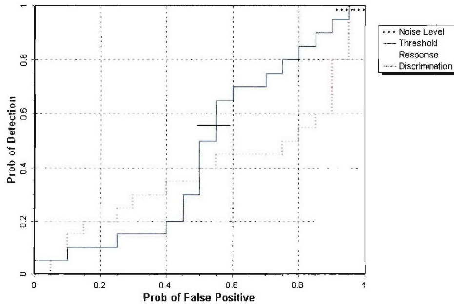
Figure 4. EM61 MKII/man-portable blind grid probability of detection for response and discrimination stages versus their respective probability of false positive for all ordnance larger than 20 mm.
