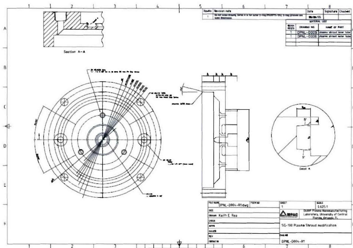
Figure 4. Orthographic drawing of the SG-100 shroud mounting plate.
