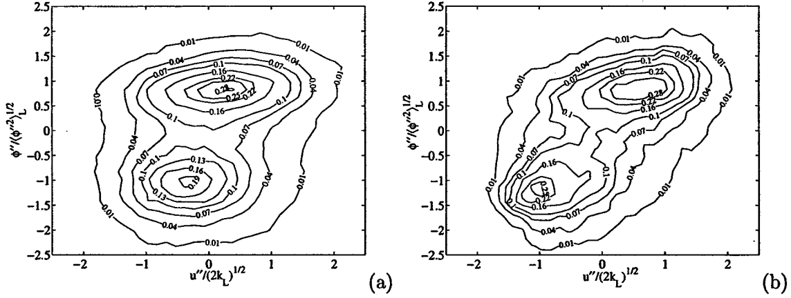
Figure 8: Mean FJDF conditional on k_L , \langle u \rangle_L , \langle \phi''^2 \rangle_L , and \langle \phi \rangle_L on the jet centerline for \langle u_1 \rangle_L = \langle u_1 \rangle (3.07 m/s) and \langle u_1 \rangle_L = 0 : (a) k_L/\langle k_L \rangle = 3.04 and \langle \phi''^2 \rangle_L/\langle \phi''^2 \rangle = 6.09 ; (b) k_L/\langle k_L \rangle = 0.64 and \langle \phi''^2 \rangle_L/\langle \phi''^2 \rangle = 6.09 . The bimodal FJDF in (b) is strongly asymmetric in u_1 , indicating large SGS flux and suggesting that mixing occurs primarily near u_1 = 0 .
