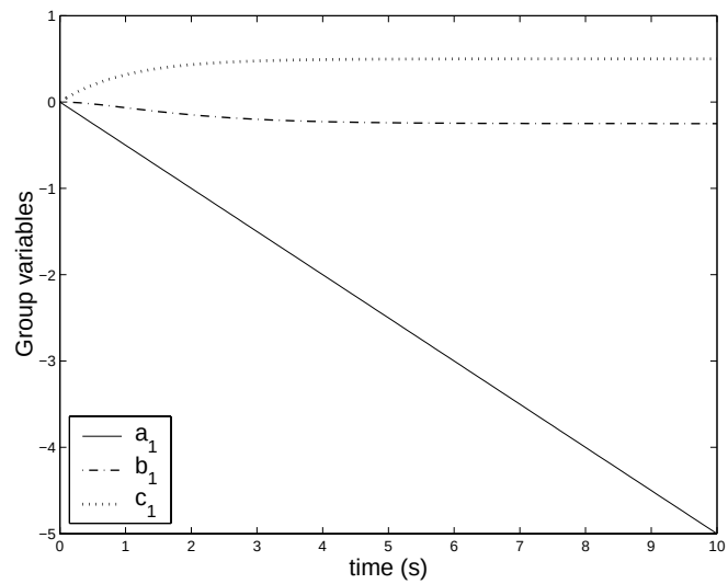
Figure 6.13: Reconstructed group motion for constant nonholonomic momentum
