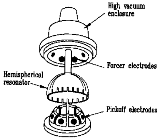
Figure 3.2: Delco HRG (Image from [50])
