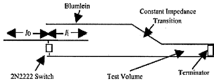
Figure 14: By retracting the center conductor to the positions in table 2, the pulse width can be selected, thereby tuning the center frequency of the Blumlein.
