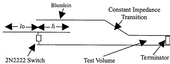
Figure 13: Concept for tuning the center frequency of the pulser.
