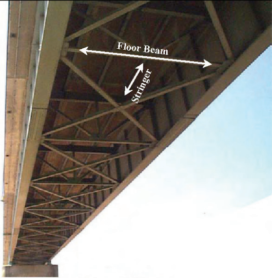
Underside View
