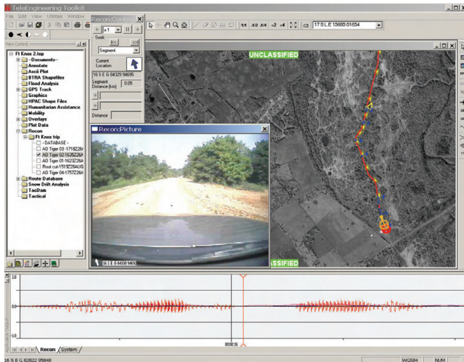
Figure 32. Output control
