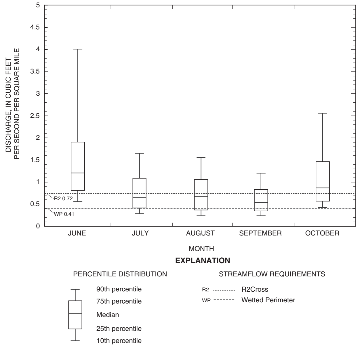
Figure 22. Distribution of median Wetted-Perimeter and R2Cross streamflow requirements for seven riffle sites on the Usquepaug–Queen River and the average distribution of the monthly mean flow during summer for the Beaver River (01117468), Branch River (01111500), and Wood River (01117800) gaging stations, Rhode Island, and the Indian Head River (01105730), Massachusetts.
