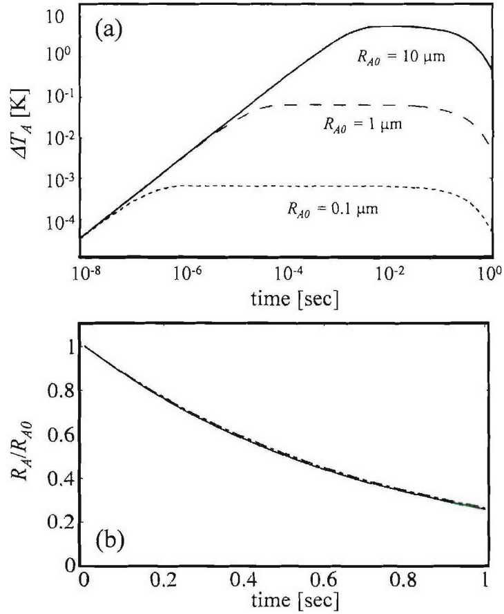
Figure 3: Aerosol temperature (a) and normalized radius (b) versus time for initial radii, R_{A0} = 0.1, 1, and 10 \mu\text{m} , and \alpha_D I = 14 \text{ kW/cm}^3 . Curves are almost indistinguishable in figure (b).
