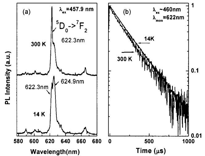
FIG. 2. (a) PL spectra of GaN:Eu under below-gap excitation (457.9 nm) at 14 and 300 K. (b) PL decay transients under below-gap excitation (460 nm) at 14 and 300 K.
