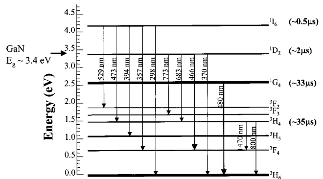
FIG. 3. Free-ion energy level diagram of \text{Tm}^{3+} ions and observed transitions in AlN:Tm. The bandgap of GaN is also indicated in the figure, along with PL lifetimes for several excited states of \text{Tm}^{3+} .
