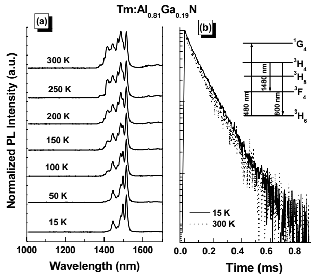
Fig. 3 a) Infrared PL spectra of \text{Al}_{0.81}\text{Ga}_{0.19}\text{N}:\text{Tm} over a temperature range from 15–300 K. The PL spectra were measured under UV Argon laser excitation (333.6–363.8) nm. b) Temperature dependent PL decay curves monitored at 808 nm. A partial energy level diagram of \text{Tm}^{3+} is also shown.
