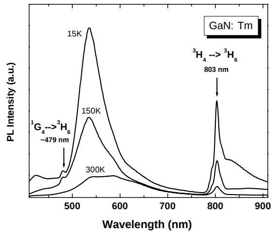
Fig. 7. PL spectra of Tm-doped GaN under above-gap excitation at 15, 150, and 300 K. The shoulder at 479 nm indicates blue emission from the ^1\text{G}_4 \rightarrow ^3\text{H}_6 intra-4f transition of \text{Tm}^{3+} .
