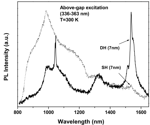
Fig. 3. Infrared PL spectra of a 7 nm GaN:Er/AlGaN SH (dotted line) and a 7 nm AlGaN/GaN:Er/AlGaN DH (solid line). The spectra were measured at 300 K using pump radiation at 336–363 nm.
